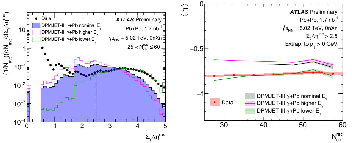
Figure 15: (left) Shown is the \Sigma_\gamma \Delta\eta^{\text{rec}} distribution for data events corresponding to N_{\text{ch}}^{\text{rec}} = 25-60 . Also, shown are the results from reconstructed event generated by DPMJET-III not corrected for detector effects utilizing the identical N_{\text{ch}}^{\text{rec}} and \Sigma_\gamma \Delta\eta^{\text{rec}} selection criteria as with experimental data for the nominal DPMJET-III and the two variations in the photon energy distribution, i.e., “higher” and “lower”. The black dashed line corresponds to the \Sigma_\gamma \Delta\eta^{\text{rec}} selection cut. (right) Shown is the \langle\eta\rangle as a function of N_{\text{ch}}^{\text{rec}} compared to the nominal truth-level yield result in DPMJET-III and two variations.
