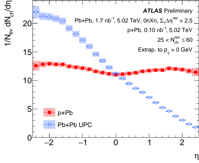
Figure 4: Shown are the charged-hadron yields as a function of \eta extrapolated to p_T > 0 GeV for Pb+Pb UPC and p+Pb collisions. The statistical uncertainties are shown as vertical lines and systematic uncertainties are shown as open boxes.
