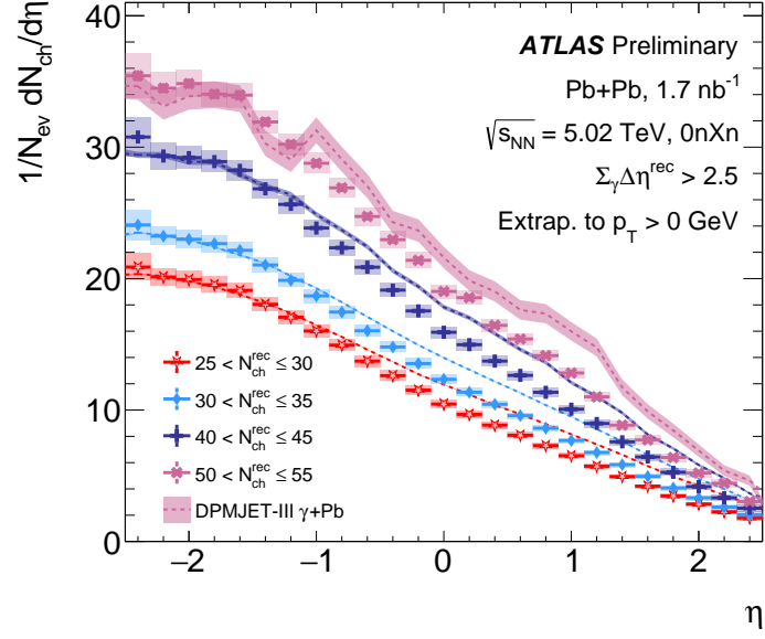
Figure 11: Shown are the charged-hadron yields as a function of \eta in different N_{\text{ch}}^{\text{rec}} bins in Pb+Pb UPC collisions extrapolated to p_{\text{T}} > 0 GeV. Vertical lines are statistical uncertainties and open boxes are systematic uncertainties. Also, shown are the truth-level yield results from reconstructed event generated by DPMJET-III utilizing the identical N_{\text{ch}}^{\text{rec}} and \Sigma_{\gamma} \Delta\eta^{\text{rec}} selection criteria as with experimental data.
