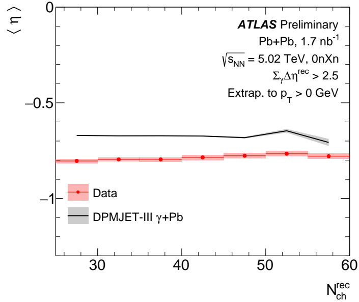
Figure 12: Shown are the calculated \langle \eta \rangle values within the window -2.5 < \eta < +2.5 of charged-hadron yields as a function of N_{\text{ch}}^{\text{rec}} in Pb+Pb UPC collisions. The charged-hadron yields are extrapolated to p_{\text{T}} > 0 GeV. Also, shown are the truth-level yield result from reconstructed event generated by DPMJET-III utilizing the identical N_{\text{ch}}^{\text{rec}} and \Sigma_{\gamma} \Delta\eta^{\text{rec}} selection criteria as with experimental data.
