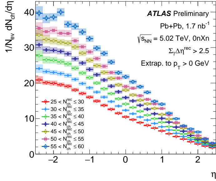
Figure 5: Shown are the charged-hadron yields as a function of \eta in different N_{\text{ch}}^{\text{rec}} bins in Pb+Pb UPC collisions extrapolated to p_T > 0 GeV. Vertical lines are statistical uncertainties and shaded boxes are systematic uncertainties.
