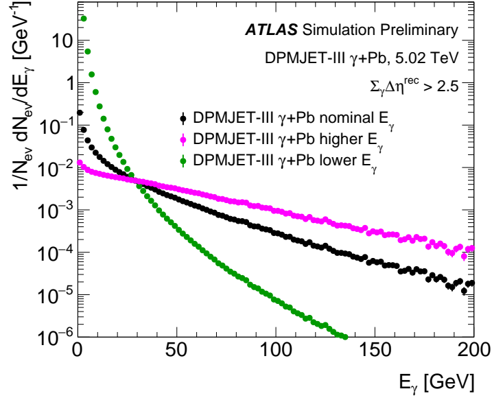
Figure 14: Shown are the DPMJET-III truth photon energy distribution for events with the generator level \Sigma_\gamma \Delta\eta^{\text{rec}} > 2.5 selection and no selection on N_{\text{ch}}^{\text{rec}} . Additionally, two re-weightings of the photon energy distribution are shown, referred to as “higher” and “lower”, that increase (decrease) the relative contribution of high-energy photons.
