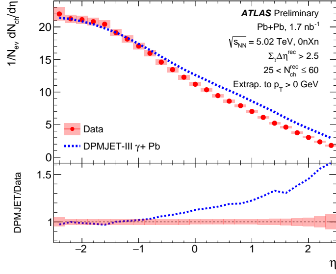
Figure 9: Shown are the charged-hadron yields as a function of \eta in Pb+Pb UPC data extrapolated to p_T > 0 GeV. Also, shown are the truth-level yield result from reconstructed event generated by DPMJET-III utilizing the identical N_{ch}^{rec} and \sum_{\gamma} \Delta\eta^{rec} selection criteria as with experimental data. The bottom panels show the ratio of DPMJET-III to data.
