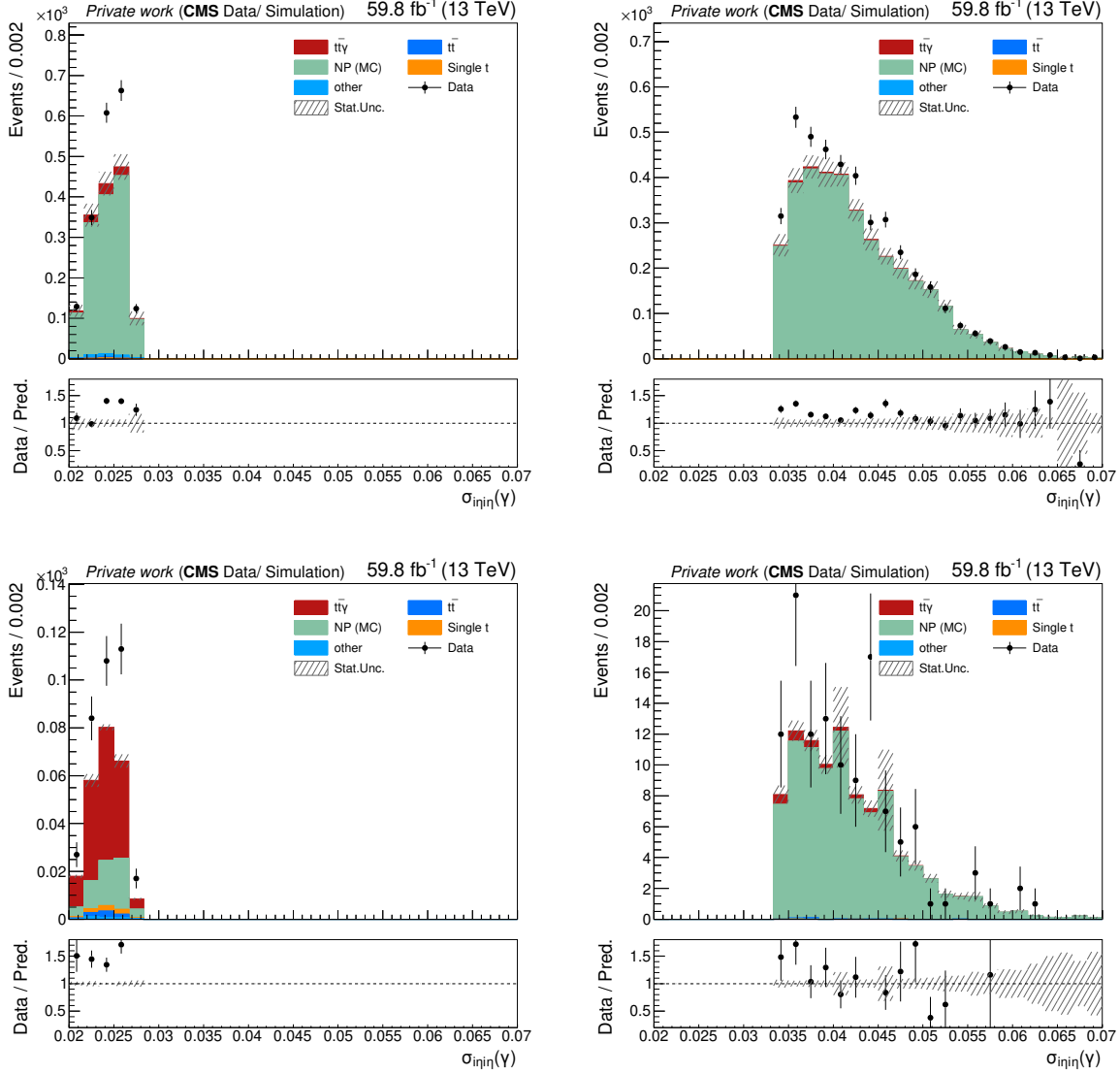
Figure 3.17: Distribution of the \sigma_{\text{inj}\eta} in the A (lower left), B (lower right), C (upper left), and D (upper right) regions used for the nonprompt photon estimation, in 2018, for photons in the EE. The positions of each figure reflect the scheme of figure 3.15. "NP (MC)" refers to the nonprompt photon contribution taken from simulation. Regions B and D, the sidebands of the \sigma_{\text{inj}\eta} cut, show good agreement between data and simulation, while regions A and C which are enriched in genuine photon events show an excess of data, same as observed in section 3.4.
