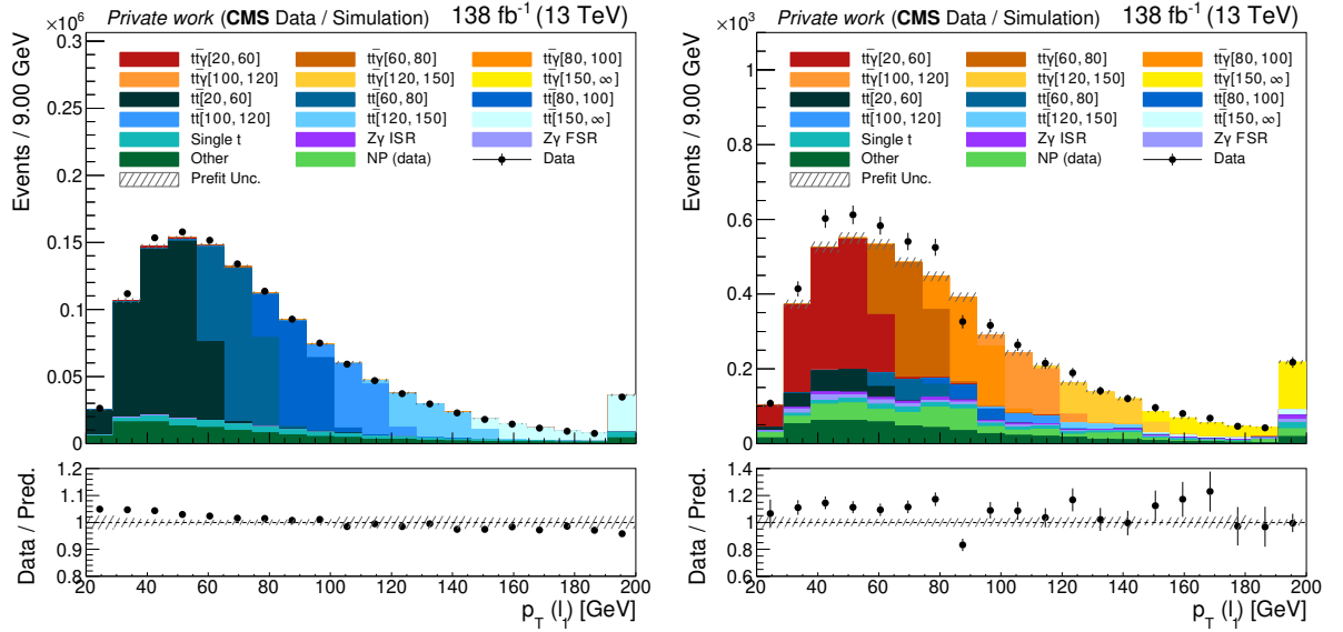
Figure 3.37: Distribution of the p_T(\ell_1) for the t\bar{t} region (left) and the SR (right), for full Run 2 data, pre-fit. The different generator-level bins of p_T(\ell_1) for t\bar{t} ( t\bar{t}\gamma ) are shown in different shades of blue (orange), from dark to light.
