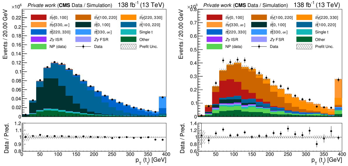
Figure 3.41: Distribution of the p_{T, \text{top}} for the t\bar{t} region (left) and the SR (right), for full Run 2 data, pre-fit. The different generator-level bins of p_{T, \text{top}} for t\bar{t} ( t\bar{t}\gamma ) are shown in different shades of blue (orange), from dark to light.
