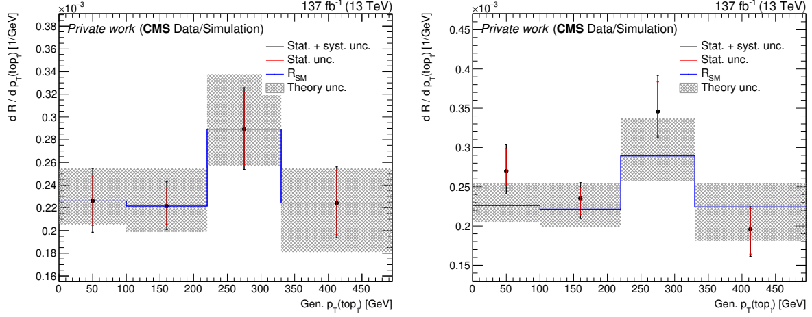
Figure 3.40: Expected (left) and observed (right) unfolded distributions of the ratio between t\bar{t}\gamma and t\bar{t} as a function of generator-level p_{T, \text{top}} .
