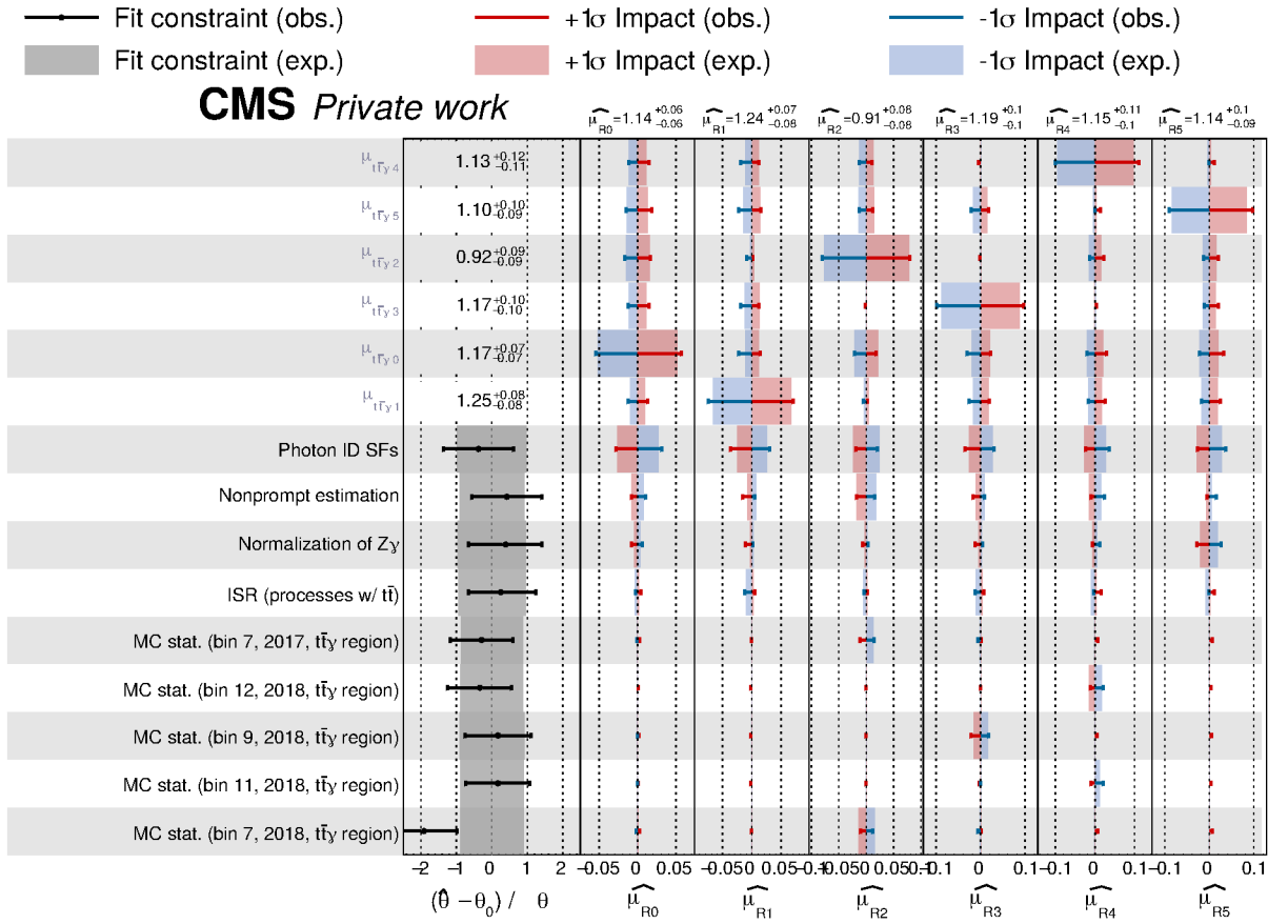
Figure 3.39: Expected and observed impacts of the leading systematic uncertainties on the different ratio parameters.
