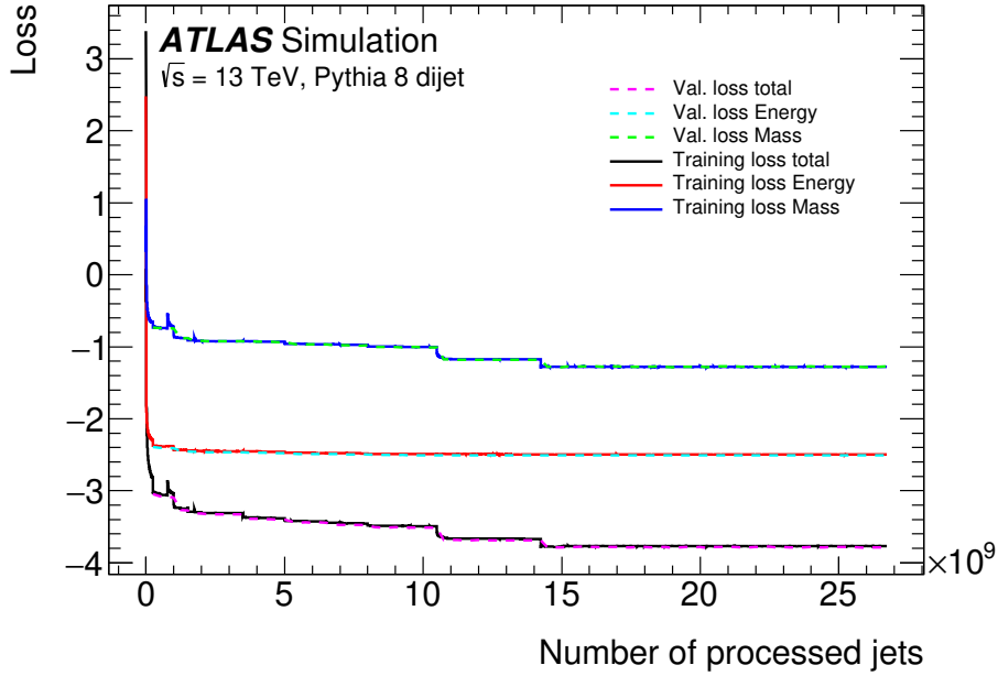
Figure 3: The loss evolution for the training (plain lines) and validation (dotted lines) data samples. The different spikes and drops correspond to the transitions between training steps (see Table 3) and are due to the variations of the loss function.
