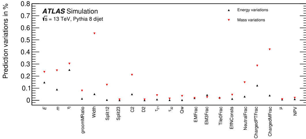
Figure 14: The variation of the energy (upward triangles) and mass (downward triangles) predictions when input features are varied (see the text for details).
