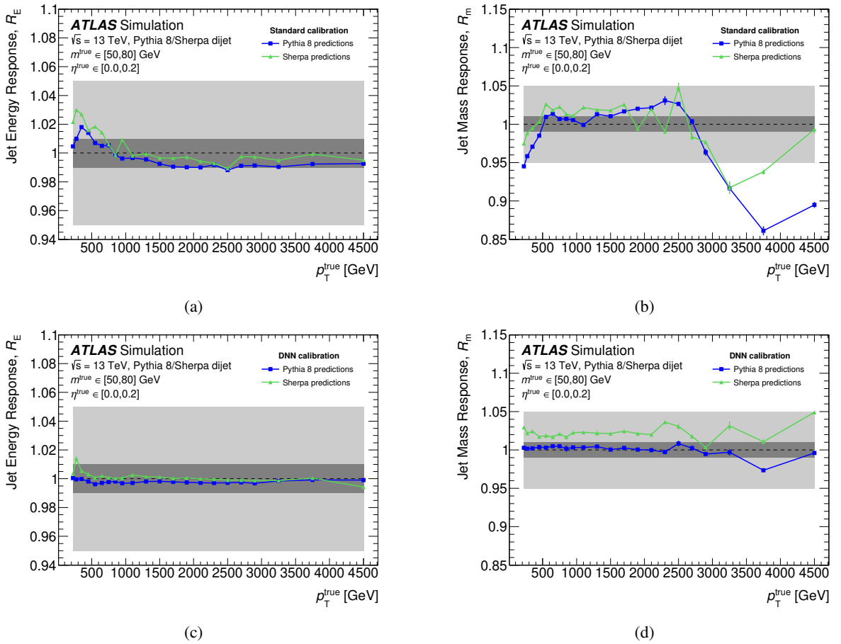
Figure 13: Jet energy and mass responses versus p_T^{\text{true}} calibrated with (a, b) the standard calibration and (c, d) with the DNN predictions for a dijet data sample generated with PYTHIA (squares) or SHERPA (triangles). The horizontal bands represent 1% (dark) and 5% (light) up and down divergences from closure.
