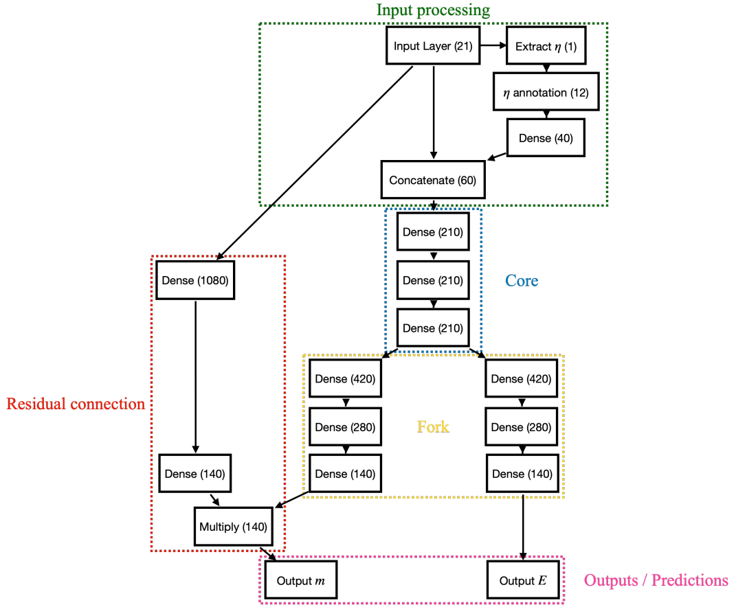
Figure 2: The architecture of the DNN.
