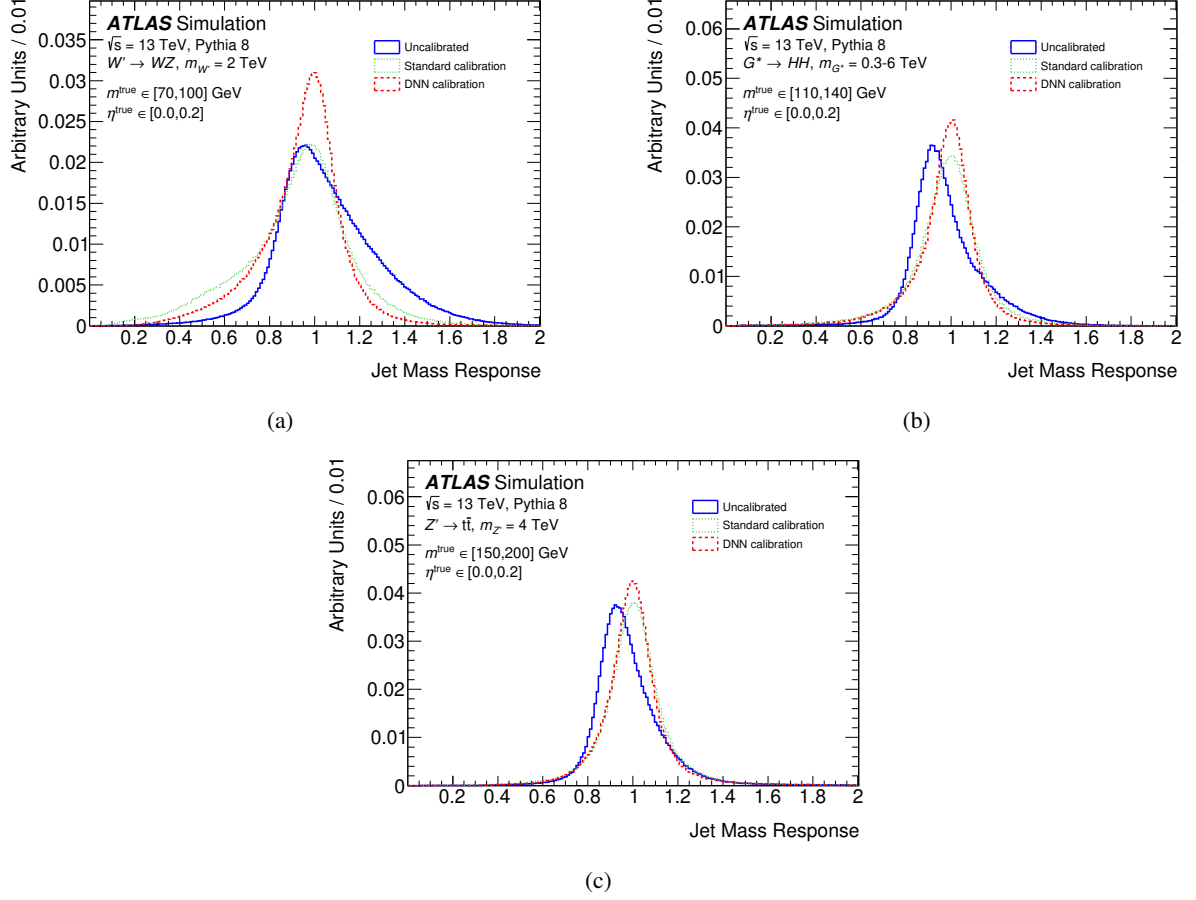
Figure 7: (a) Boosted W/Z, (b) Higgs boson and (c) top-quark mass response distributions (normalised to unity) for different calibrations: uncalibrated (plain line), standard calibration (dotted line) and DNN calibration (dashed line).
