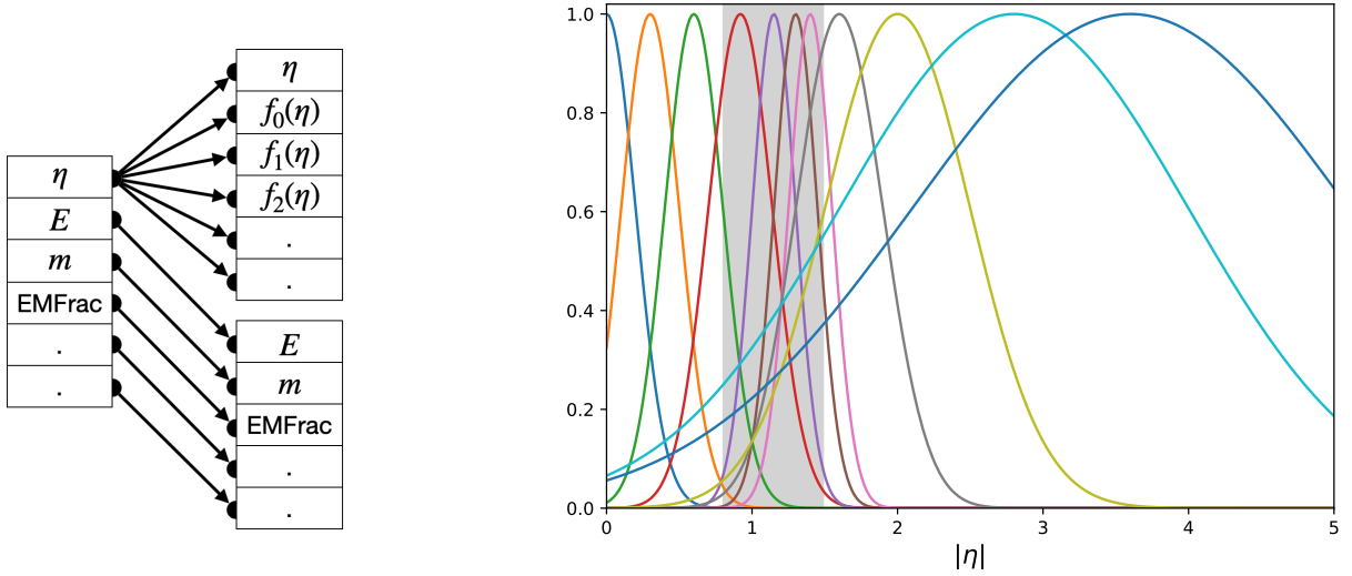
Figure 1: The principle of the \eta annotation (left) and the various f_i(\eta) functions (right). The vertical shaded band on the right plot marks the calorimeter transition region.
