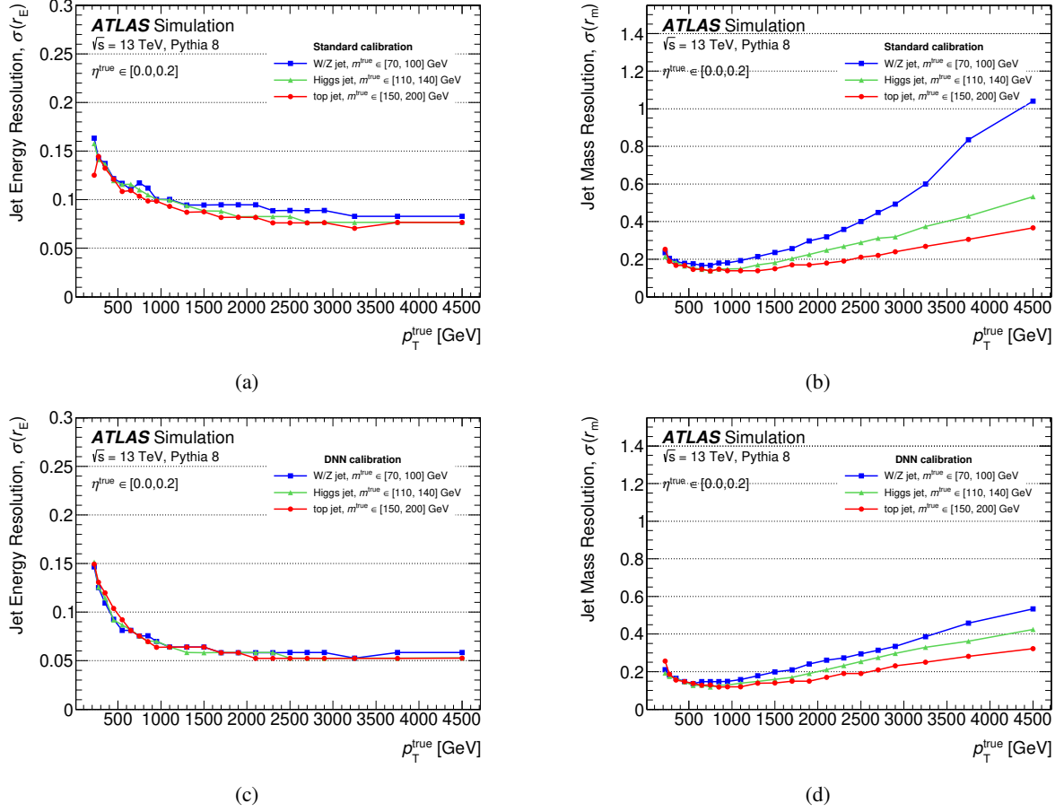
Figure 9: Boosted W/Z , top-quark and Higgs boson jet energy (left) and mass (right) resolutions as a function of p_T^{\text{true}} for different calibrations: (a, b) standard calibration and (c, d) DNN calibration.
