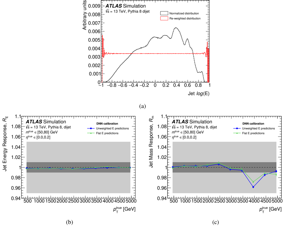
Figure 10: Normalised distributions of (a) the jet energy before (black) and after (red) re-weighting. And the corresponding (b) jet energy and (c) mass responses obtained with the DNN calibration as a function of p_T^{true} for these two energy distributions, the unweighted distribution (squares) (as used for training) and the flat-energy weighted distribution (triangles). The horizontal bands represent 1% (dark) and 5% (light) up and down divergences from closure.
