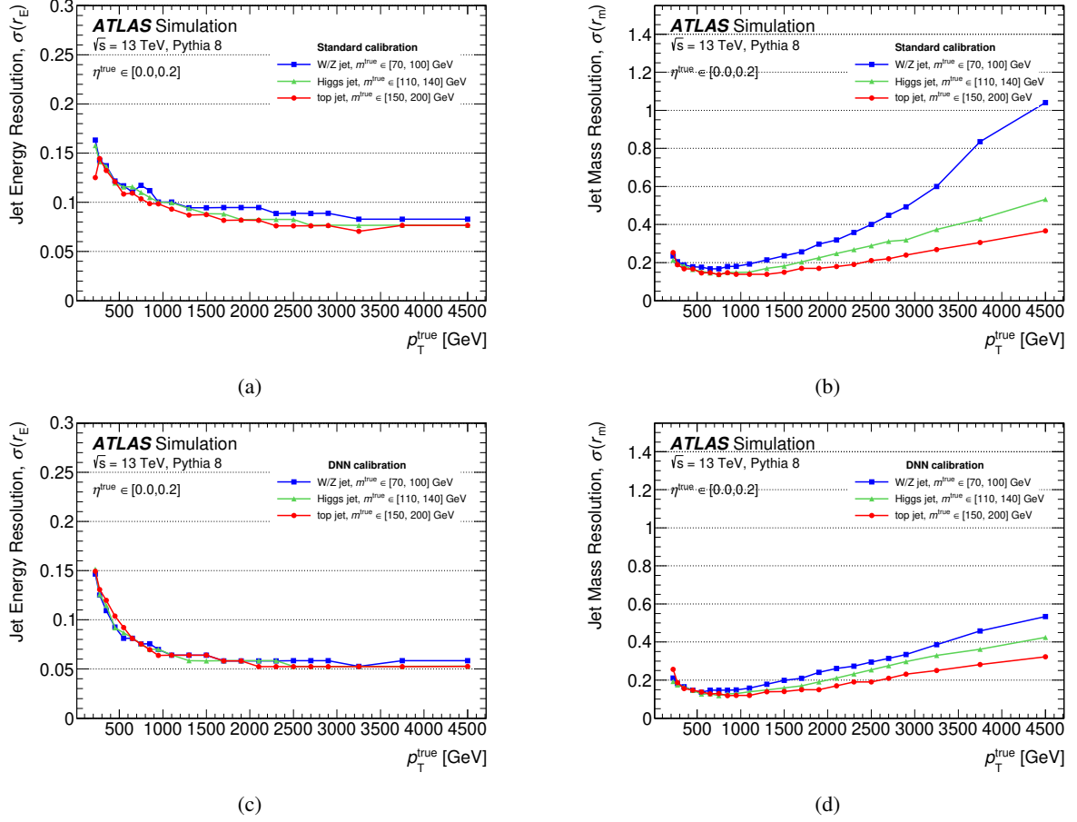
Figure 9: Boosted W/Z, top-quark and Higgs boson jet energy (left) and mass (right) resolutions as a function of p_T^{\text{true}} for different calibrations: (a, b) standard calibration and (c, d) DNN calibration.
