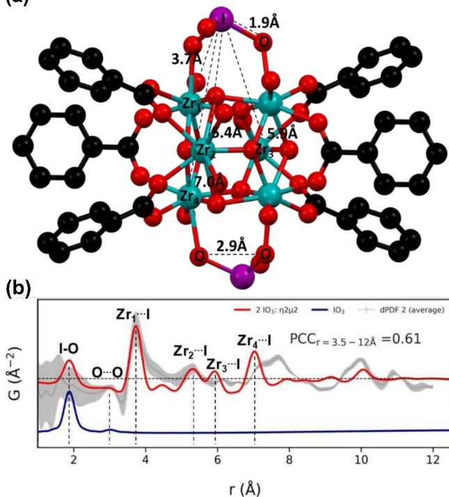
Figure 4. (a) MOF-808 node with bridging iodate ions. (b) Simulated differential pair distribution function (dPDF) of this DFT model (red trace) overlaid atop experimentally obtained dPDF of iodate-loaded MOF-808 from X-ray total scattering data (grey trace) alongside the PDF of unbound iodate (blue trace).
