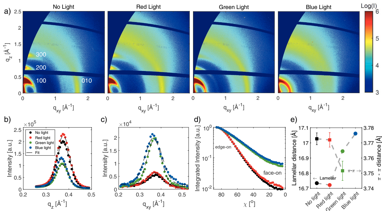
Figure 3. a) GIWAXS data with Ewald sphere correction of P3HT slot-die coated on top of silicon with varying light treatments, with ( q = 4\pi \sin(\theta)/\lambda , where \theta is half the scattering angle, and \lambda is the X-ray wavelength). Lamellar stack (100) and \pi-\pi stack (010) signals are indicated with white text in the left panel. The colour scale is logarithmic and equal for the four data sets shown. b) Out-of-plane ( q_z ) line integration of lamellar peak and Gaussian fit. c) In-plane ( q_{xy} ) line integration of lamellar peak and Gaussian fit. d) Integrated lamellar signal as a function of \chi , where 0^\circ corresponds to in-plane and 90^\circ corresponds to out-of-plane orientation of the lamellar stacking direction, indicating face-on and edge-on orientation of the polymer planes with respect to the substrate. e) Out-of-plane lamellar and in-plane \pi-\pi packing distances for the four treatments. Lamellar distances are indicated with circular symbols (error bars are smaller than the symbols) and refer to the left axis, whereas the \pi-\pi distances are indicated with squares and refer to the right axis. As a consequence of not having any in-plane \pi-\pi stacking peak in the blue light sample (see Figure S5, Supporting Information), no value is shown here.
