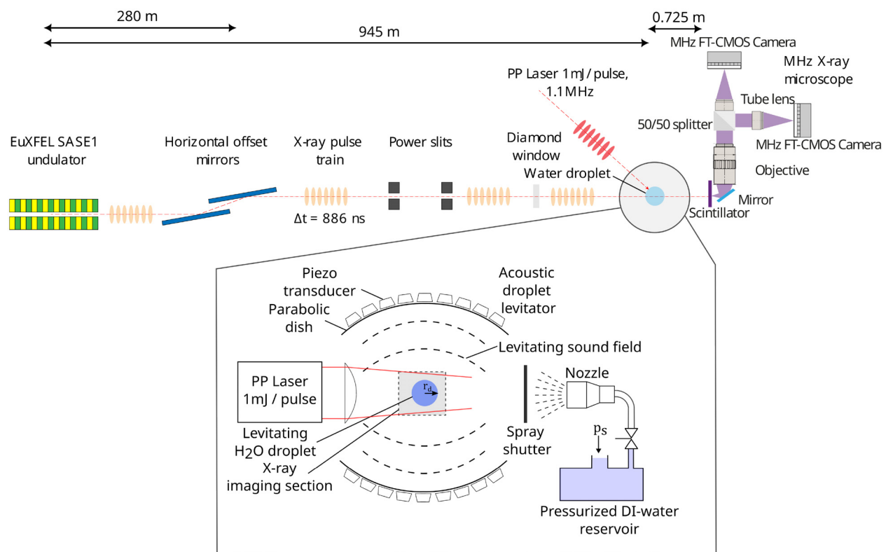
FIG. 1. Schematics of experimental arrangement with direct beam illumination at SPB/SFX instrument at EuXFEL (top) and sample setup (bottom). A water spray is produced through a nozzle, and a water droplet (of a specific size) is trapped in the standing wave field of the acoustic levitator. A mildly convergent laser pulse explosively fragments the quiescent droplet. The time-resolved dynamics are recorded in the x-ray imaging section.
