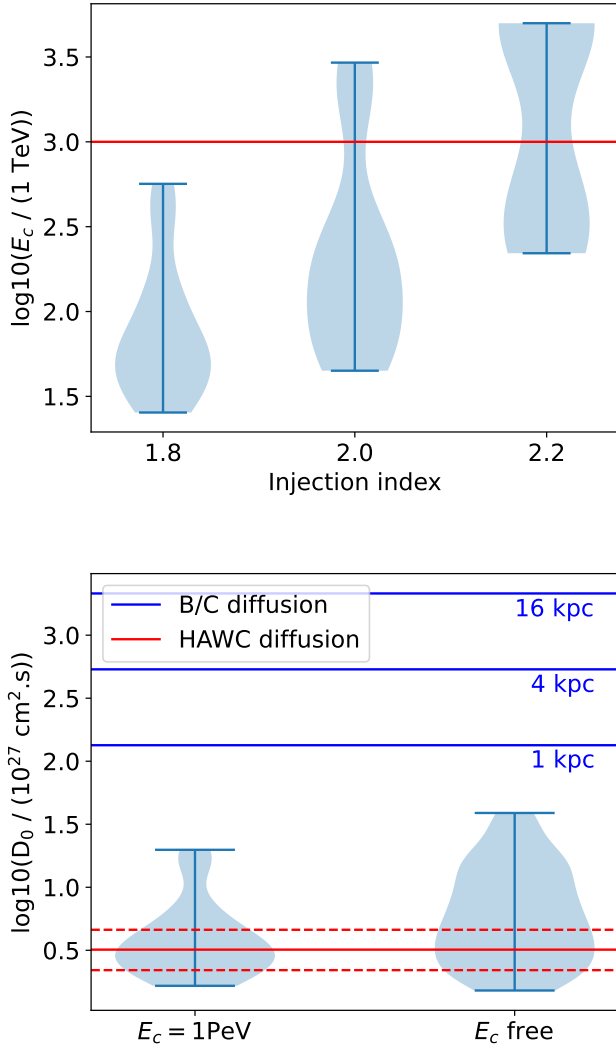
Fig. 12. Distribution of models with p -value > 0.003 , presented as a violin plot, illustrating the kernel probability density. The width of the shaded area represents the proportion of number of fits located at these positions. The upper and lower bars represent the maximum and minimum values. Top: Fitted energy cut-off distribution as a function of injection index for the combined H.E.S.S. and HAWC dataset. The red horizontal line shows the value of energy cut-off chosen for the fixed E_c fit. Bottom: distribution of the fitted diffusion coefficient in the case of E_c = 1 PeV and E_c left free to vary, for a combined fit to H.E.S.S. and HAWC data. Solid lines indicate the value ranges for the B/C diffusion coefficient and the statistical uncertainty of HAWC diffusion coefficient obtained in Abeysekara et al. (2017a).
