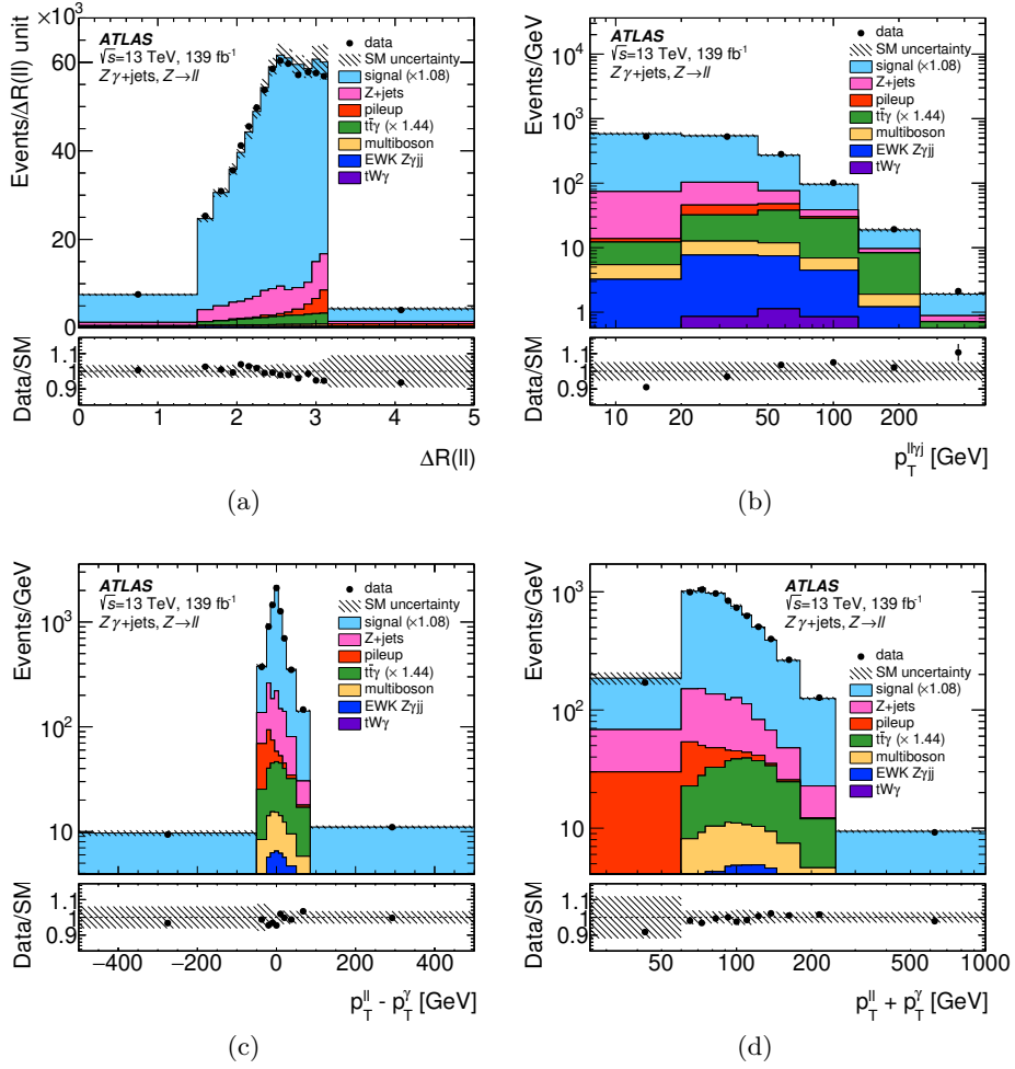
Figure 3. The measured (a) \Delta R(\ell, \ell) , (b) p_T^{\ell\ell\gamma} , (c) p_T^{\ell\ell} - p_T^\gamma , and (d) p_T^{\ell\ell} + p_T^\gamma distribution (dots) in the signal region. The error bars represent the data statistical uncertainty; for most of the points, the error bars are smaller than the marker size and, thus, not visible. The MC simulation of the signal from SHERPA 2.2.11 (blue histograms) and various backgrounds are also included. The signal and background distributions are stacked to produce the figures. The variable bin width is taken into account in the vertical scale. The lower part of each figure shows the ratio of the data to the expected total SM distribution. The hatched band represents the statistical and systematic uncertainties of the SM background yields added in quadrature, excluding theory uncertainties of the signal.
