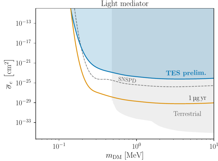
Figure 1: Terrestrial parameter space for DM-electron scattering with a light mediator in the \sim MeV mass range dependent on the DM-electron scattering cross section \sigma_e . The blue area shows the preliminary projection (20 ng hr) for our TES based only on intrinsic measurements (for ALPS II). The dotted gray line describes the parameter space covered by SNSPD measurements (774 ng hr) with the projection for a larger exposure of SNSPDs in orange (from [13]). The shaded gray area represents other terrestrial constraints.
