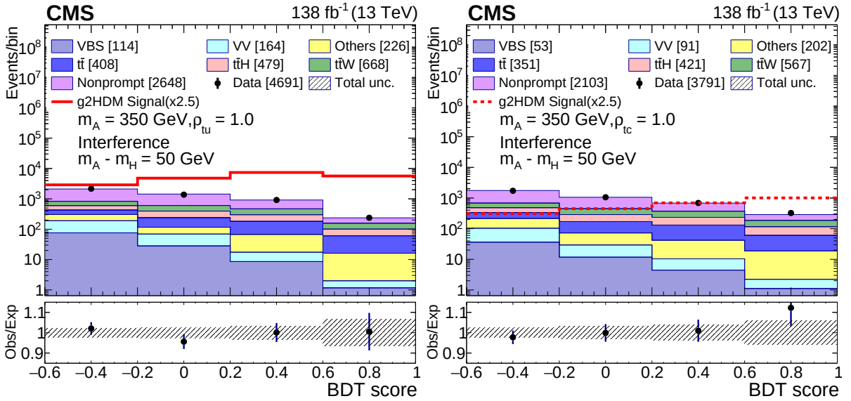
Figure 3: Post-fit distributions of the BDT discriminants combining the categories e^\pm e^\pm , \mu^\pm \mu^\pm , and e^\pm \mu^\pm , for m_A = 350 GeV with \rho_{tu} = 1.0 (left), and \rho_{tc} = 1.0 (right) with the A-H interference. The numbers in square brackets represent the yields for each sample. The uncertainty bars on the points represent the statistical uncertainties in the data. Beneath each plot the ratio of data to predictions is shown. The uncertainty bars in the ratio plots include statistical uncertainties in the data and the total uncertainty in the background predictions, and the hatched bands represent the total uncertainty in the background predictions.
