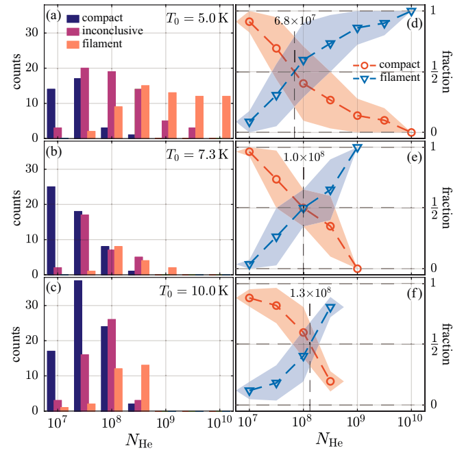
FIG. 3. Mapping structure formation as a function of the droplet size. The counts (a)–(c) and fractions (d)–(f) of the identified compact and filament xenon nanostructures for T_0 = 5 K, 7.3 K, and 10 K (from top to bottom). Structures that could not be assigned to either categories are categorized as inconclusive (see Fig. S5 in SM [39]) and serve as identification error for the fraction diagrams.
