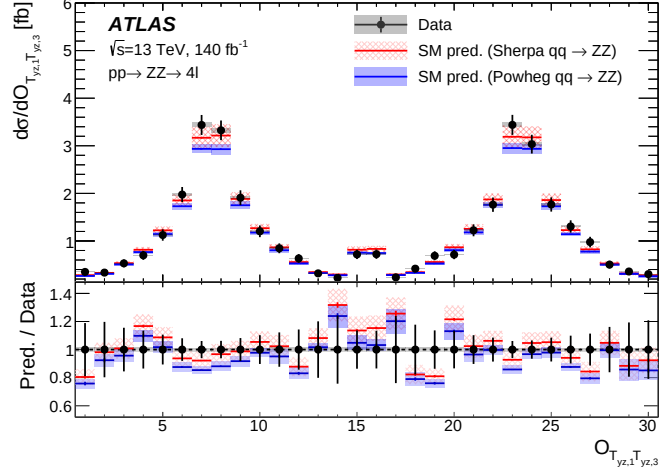
Figure 8: Unfolded differential cross-section as a function of the Optimal Observable O_{T_{yz,1}T_{yz,3}} . The grey, red and blue uncertainty bands represent the respective systematic uncertainties in the measured unfolded cross-section and predicted particle-level cross-sections, where the q\bar{q} \rightarrow ZZ contribution is predicted using either the SHERPA or POWHEG generators. The vertical error bars represent the total uncertainties in the measured differential cross-section.
