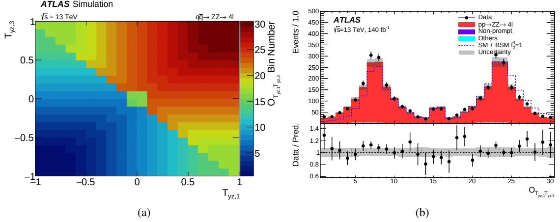
Figure 5: (a) The 2D \rightarrow 1D mapping and (b) the detector-level measurement of the OO O_{T_{yz,1}T_{yz,3}} . The measured distribution is compared with the SM signal prediction and the total background. The ‘Others’ category includes the contribution from t\bar{t}Z and VVZ processes. The non-prompt background is estimated by using the fake-factor method. The grey band represents the effect of the total theoretical and experimental uncertainties for the detector-level predictions, and the vertical error bars on data represent the statistical uncertainties. The effect of CP-odd BSM coupling is also represented by the dashed histogram.
