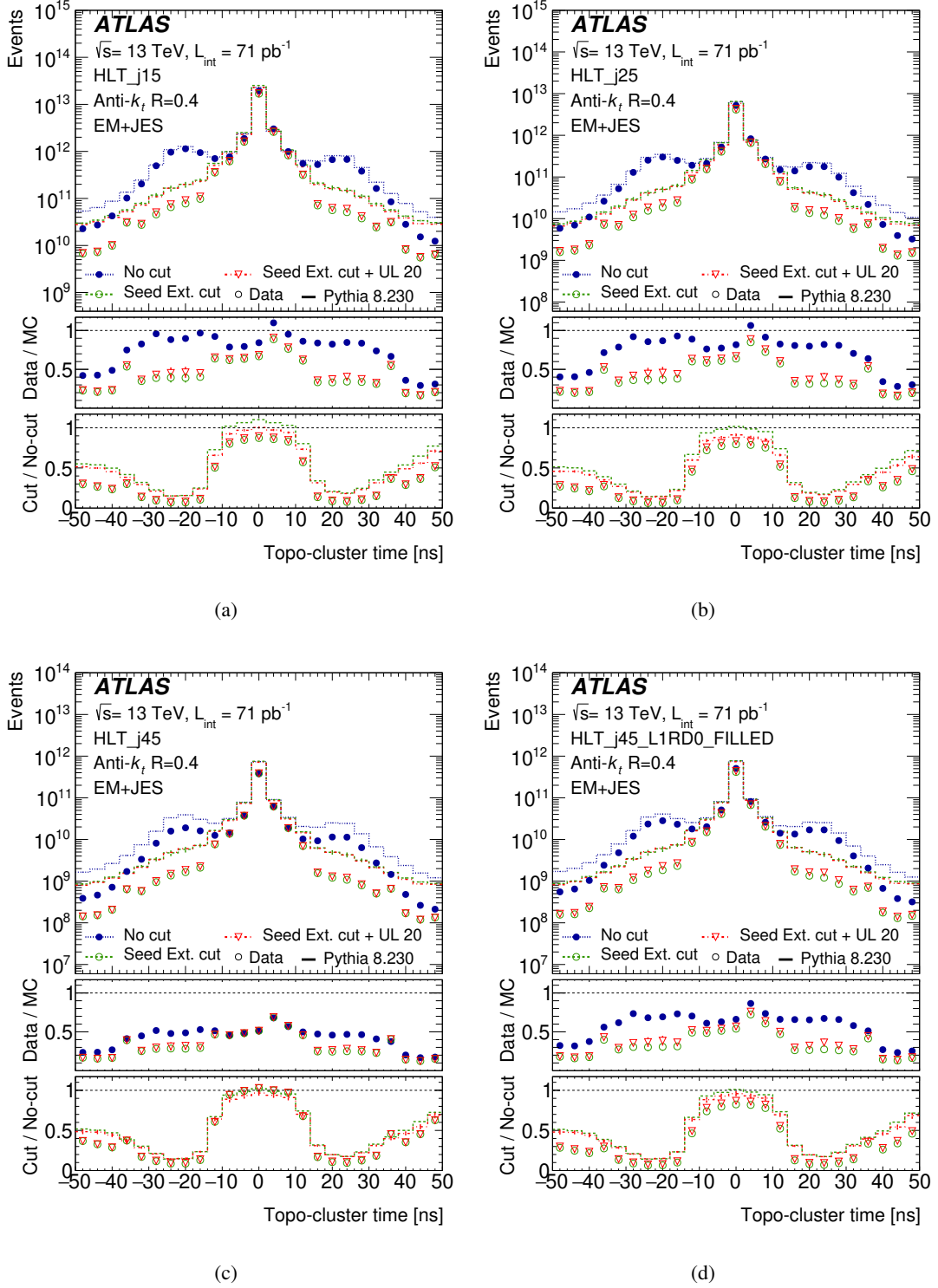
Figure 13: Topo-cluster time spectrum in data and MC selected multi-jet events. Four triggers are compared: (a) HLT_j15, (b) HLT_j25, (c) HLT_j45, and (d) HLT_j45_L1RDO_FILLED. The error bars convey the statistical and luminosity uncertainties. Uncertainties in the cut / no-cut ratios are obtained by splitting the available sample into subsamples and recomputing the cut / no-cut ratio for each subsample. The root-mean-square of the distribution of the ratio is used to estimate the ratio's uncertainty. The luminosity uncertainty does not apply to the cut / no-cut ratio.
