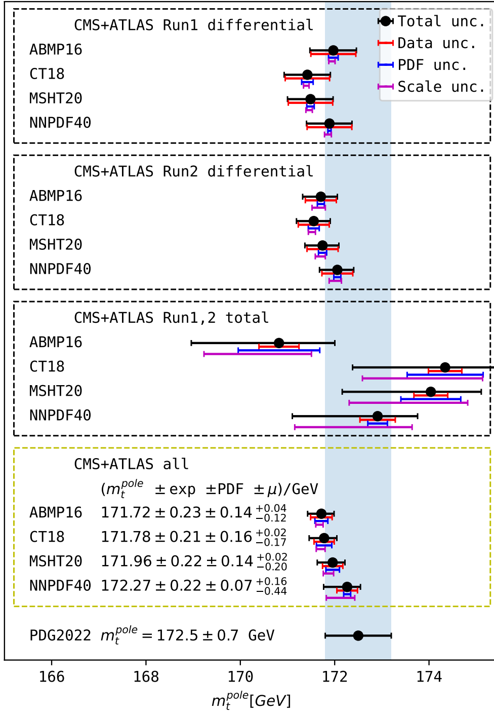
Figure 17. Summary of the m_t^{\text{pole}} values extracted from Run1 and Run2 measurements of differential and total t\bar{t} + X cross sections (the first two insets are the same as the lowest insets in Fig. 16.).
