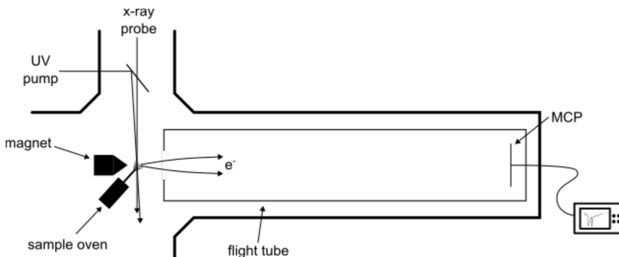
Figure 3: Sketch of the experimental setup. A UV-pump x-ray probe scheme was used in all experiments. Photo- and Auger-Meitner electrons were collected using a magnetic bottle time-of-flight spectrometer.
