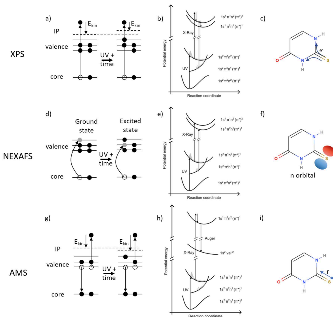
Figure 2: Probing schemes for different x-ray spectroscopic methods addressed in this review and pictograms on how they relate to the molecular problem. In the first column, electron balls schemes are shown depicting the x-ray probing mechanism for ground and excited state molecules. The middle column shows sketches of potential energy surfaces. The right column shows the molecules and related observables.
