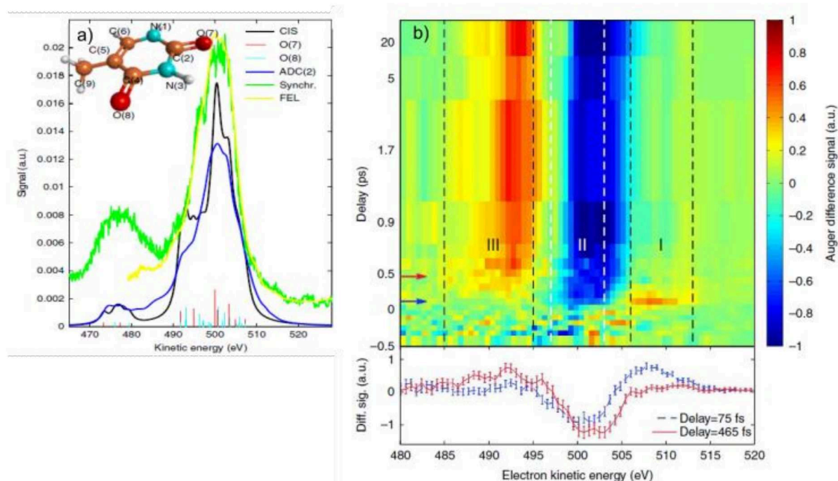
Figure 6: a) Static Auger-Meitner spectra of thymine. b) Delay-dependent false-color map of the difference between ground-state and UV-excited AM spectra of thymine. Material from figs. 2 and 3 in ref. [86] without changes.
