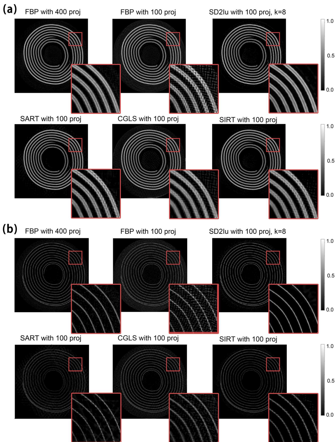
Fig. 7 Two example XRD-CT reconstruction images: (a) chemical image corresponding to the NMC532 phase, (b) chemical image corresponding to the Cu phase. All SD2I results are using k factors equal to 8. The image sizes are 547 \times 547 . The SD2I and FBP results are reconstructed from the sinogram size as 547 \times 100 . The ground truth is obtained by the CGLS reconstruction of the 547 \times 400 sinogram.
