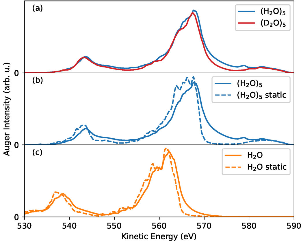
FIG. 6. Calculated Auger electron spectrum. (a) Comparison for the deuterated [(D_2O)_5] and non-deuterated [(H_2O)_5] water pentamer in a tetrahedral arrangement. (b) Auger spectrum for the water pentamer [(H_2O)_5] . (c) Auger spectrum for isolated water ( H_2O ). The dashed lines in panels (b) and (c) show instantaneous spectra at t = 0 , i.e., without taking into account the effect of core-hole-lifetime nuclear dynamics.
