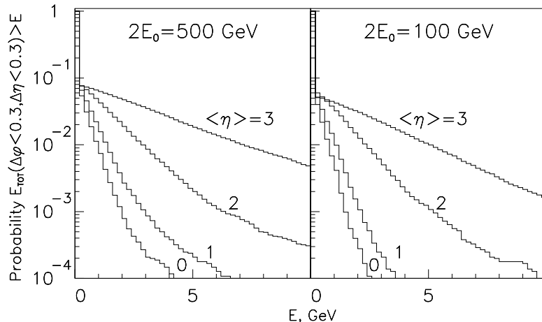
Figure 20: Probability to have the energy flow into \Delta\phi \times \Delta\eta = 0.3 \times 0.3 cell above some threshold (abscissa value) for 4 pseudorapidity points: \eta = 0, 1, 2, 3 . The energy of symmetrical \gamma\gamma is 500 GeV (left) and 100 GeV (right).
