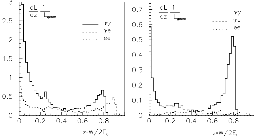
Figure 14: Luminosity spectra for the “super TESLA(4)” parameters (see the text). Left figure - without the deflection; right - \gamma\gamma collisions with the magnetic deflection.
