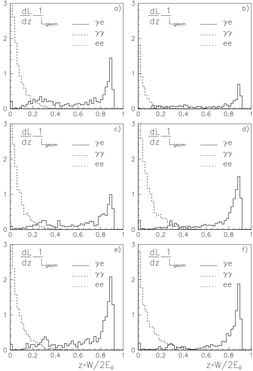
Figure 13: Spectral \gamma luminosity in the scheme with the same vertical deflection as for \gamma\gamma collisions (fig. 11) for beam parameters presented in Tables 2, 3. (Figs. 13a), b)... correspond to TESLA(1), TESLA(2)...). For additional comments see the text.
