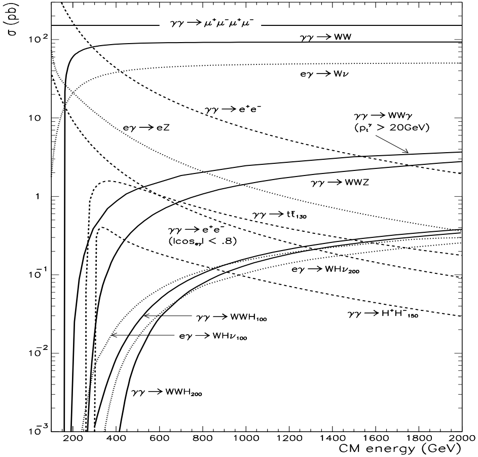
Figure 2: The cross sections of some processes in \gamma\gamma and \gamma e collisions.
