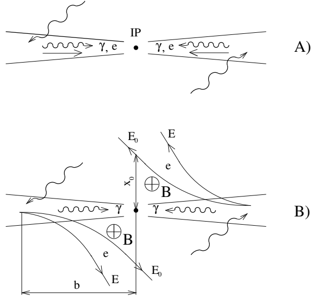
Figure 8: Two basic collision schemes: a) “without deflection”, b) “with deflection” using the sweeping magnet.
