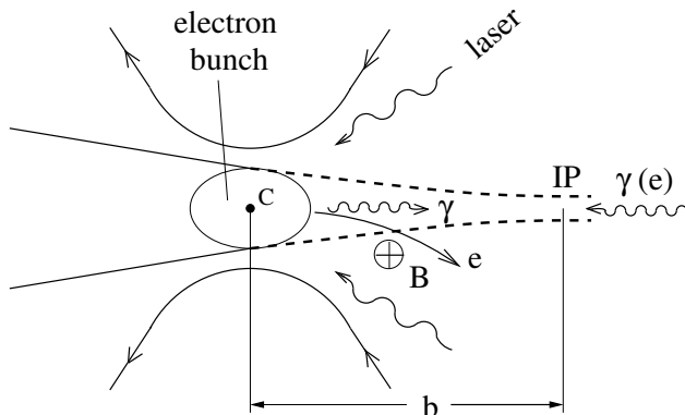
Figure 1: Scheme of a \gamma\gamma ; \gamma e collider.
