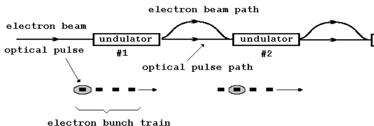
Figure 26: The scheme of multi-stage FEL amplifier. One optical pulse is amplified by a sequence of electron bunches. The peak power of the output radiation exceeds by a factor of N (number of amplification stages) the peak output radiation power of traditional single pass FEL amplifier.
