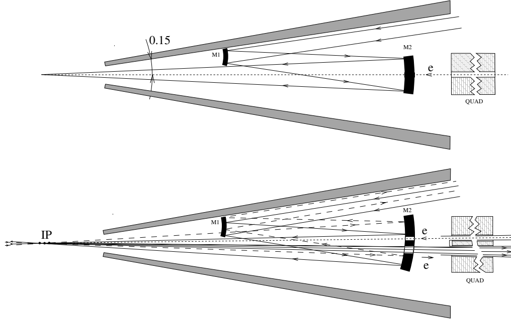
Figure 21: Layout of laser optics near the IP; upper - side view, down - top view, dashed lines - exit path of light coming from the left through one of the CP points (right to the IP), see comments in the text.
