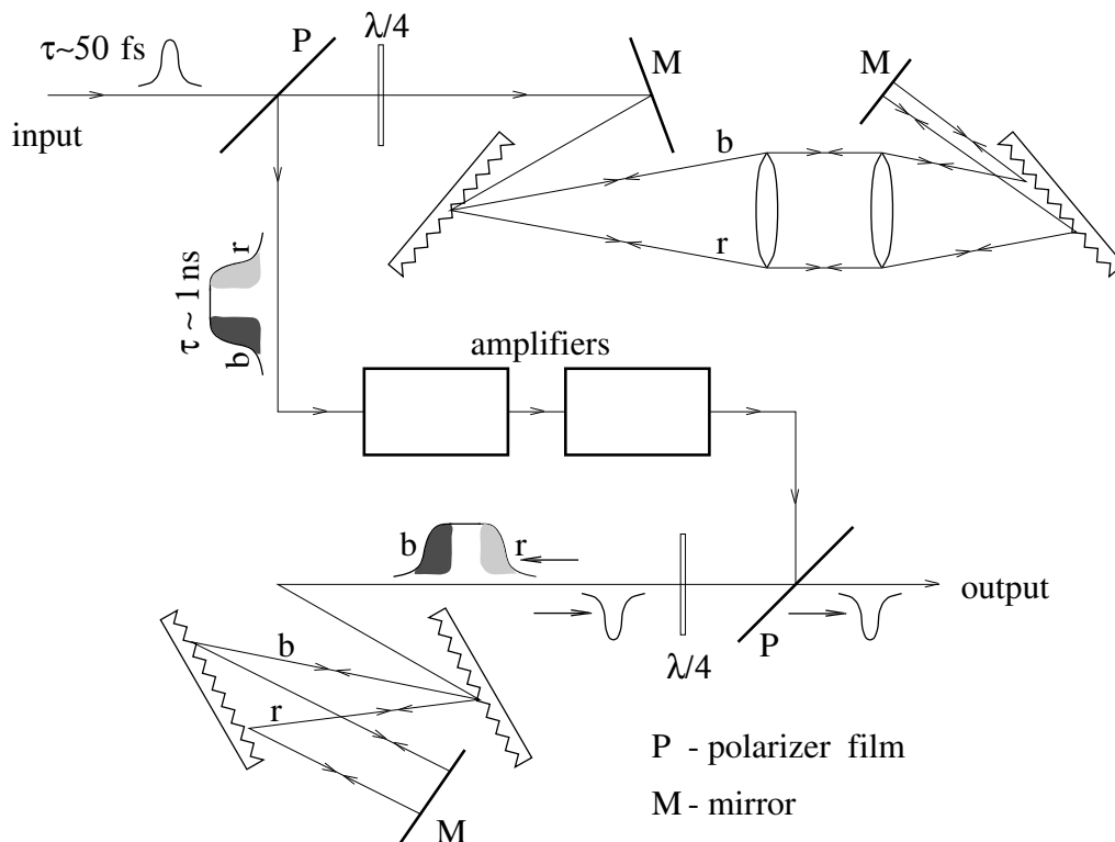
Figure 23: Chirped pulse amplification.
