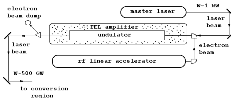
Figure 24: MOPA FEL configuration for a gamma-gamma collider.
