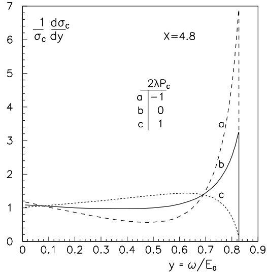
Figure 4: Spectrum of the Compton scattered photons for different polarizations of the laser and electron beams.
