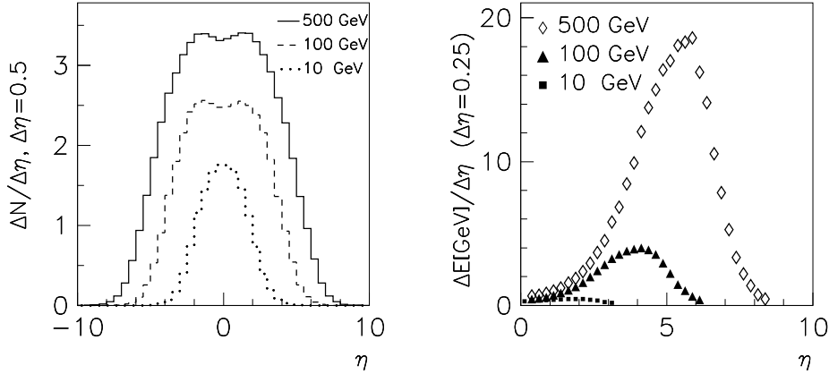
Figure 16: Distribution of particle (left) and energy flow (right) on pseudorapidity in \gamma\gamma \rightarrow \text{hadrons} events (photons have equal energies).
