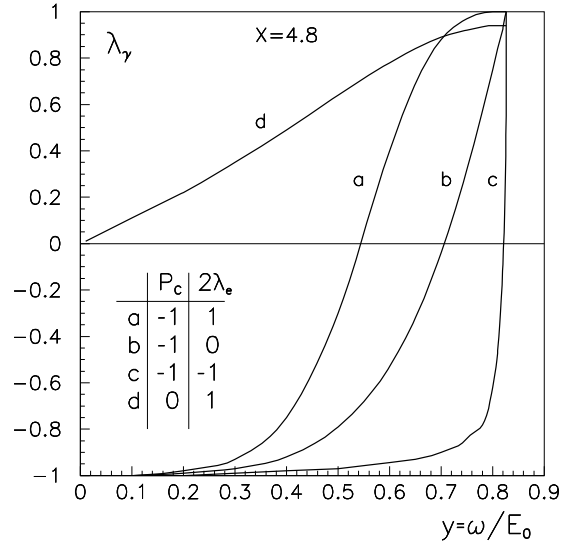
Figure 5: Mean helicity of the scattered photons.
