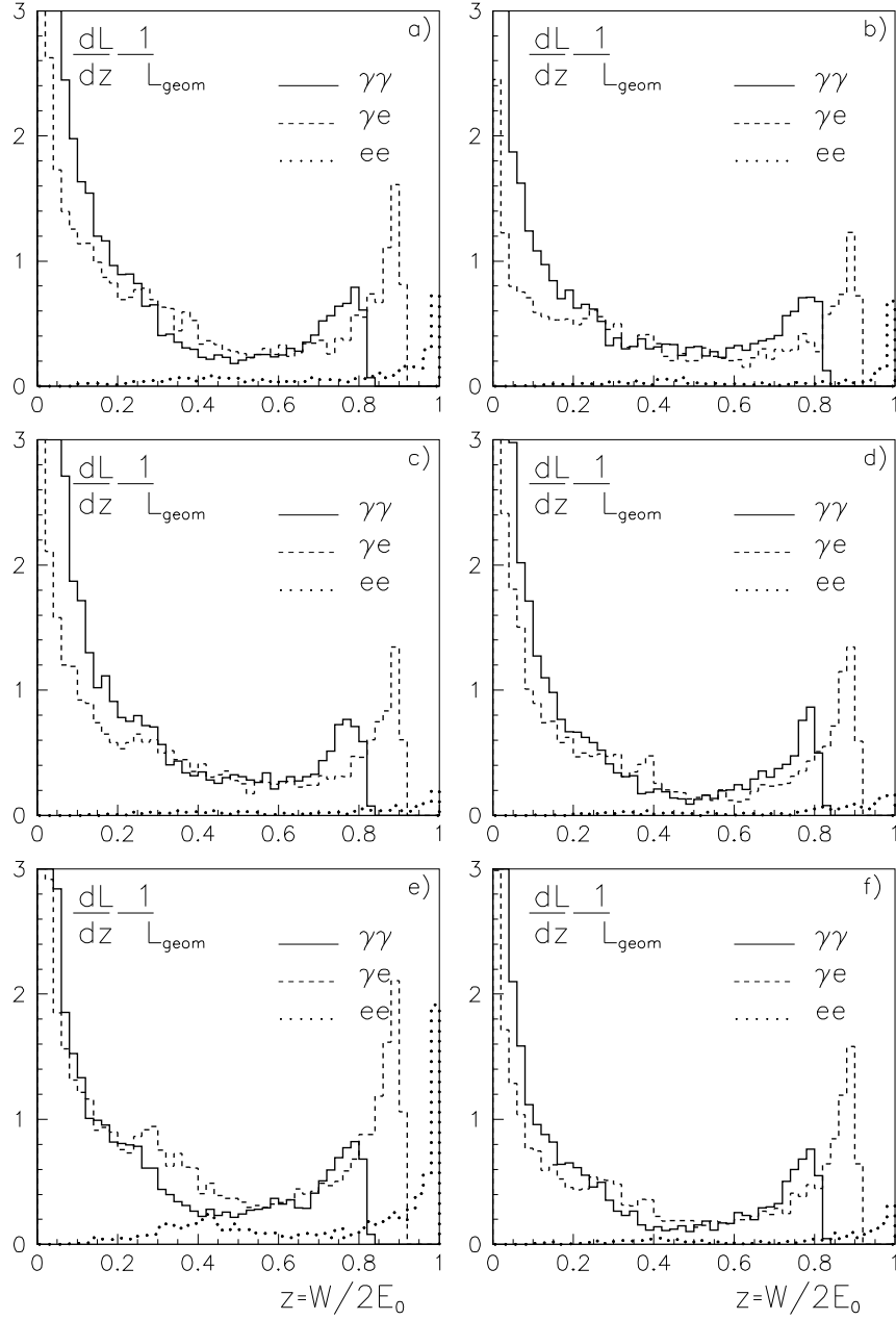
Figure 10: Luminosity spectra for the scheme without deflection for the \gamma\gamma collider parameters presented in Tables 2, 3 (Figs. 10a), b)... correspond to TESLA(1), TESLA(2)...). Luminosity distributions are normalized to the geometrical luminosity. For additional comments see the text.
