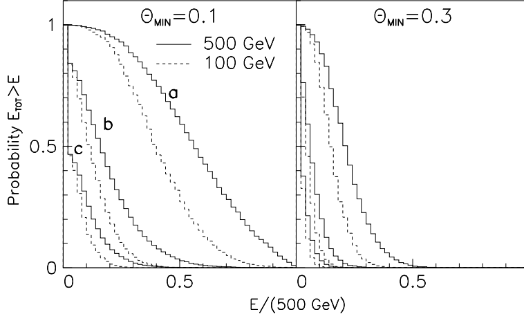
Figure 18: Probability of energy deposition in the detector above some value ( E/500 GeV) due to the process \gamma\gamma \rightarrow hadrons . The polar angle acceptance is \vartheta > 0.1 rad (left plot) and \vartheta > 0.3 rad (right plot). Curves a), b), c) correspond to 7, 2 and 0.7 hadronic events on the average per beam collision respectively. The collision energy is 500 GeV (solid line) and 100 GeV (dashed line), photons have equal energies.
