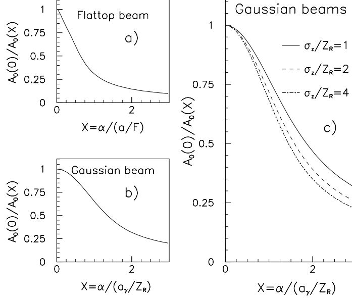
Figure 22: Dependence of the required laser flash energy on the collision angle between the laser and electron beams; (a) flattop, (b) Gaussian beams. Plots a), b) correspond to very long laser beams. Plot c) shows the same for Gaussian beams for different ratios of \sigma_z/Z_R assuming that \sigma_{L,z} = \sigma_z .
