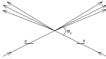
Figure 9: Crab-crossing scheme.
