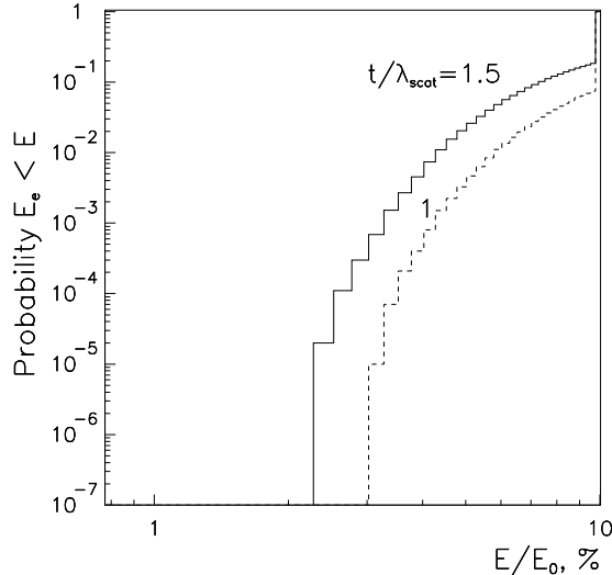
Figure 7: Probability for an electron after the conversion region to have an energy below E/E_0 .
