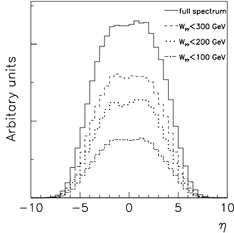
Figure 17: Distribution of particles on pseudorapidity for different ranges of \gamma\gamma invariant mass for the TESLA(1) case without deflection (see Fig. 10a).
