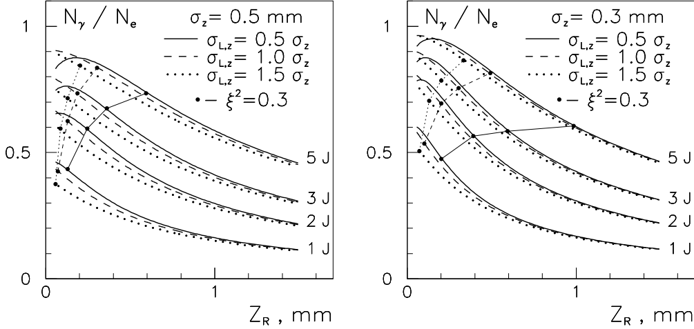
Figure 6: Conversion efficiency vs Z_R for various values of the flash energy and photon bunch length. Left figure for electron bunch length \sigma_z = 0.5 \text{ mm} (TESLA), right for \sigma_z = 0.3 \text{ mm} (SBLC).
