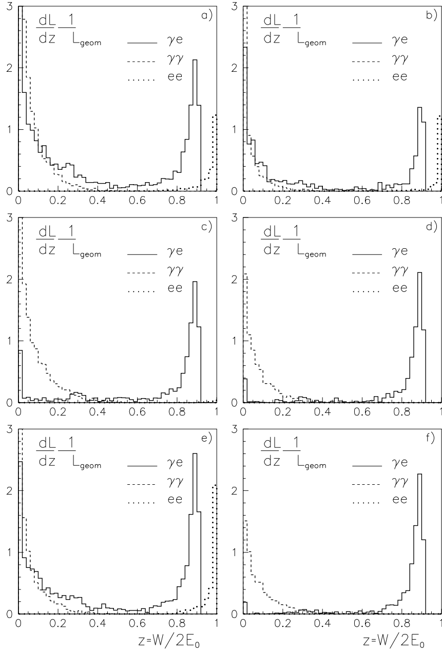
Figure 12: Spectral \gamma e luminosity in the scheme with the horizontal deflection for beam parameters presented in Tables 2, 3. (Figs. 12a), b)... correspond to TESLA(1), TESLA(2)...). For additional comments see the text.
