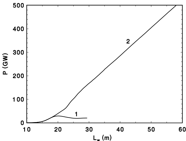
Figure 25: Output power of the FEL amplifier versus undulator length.
