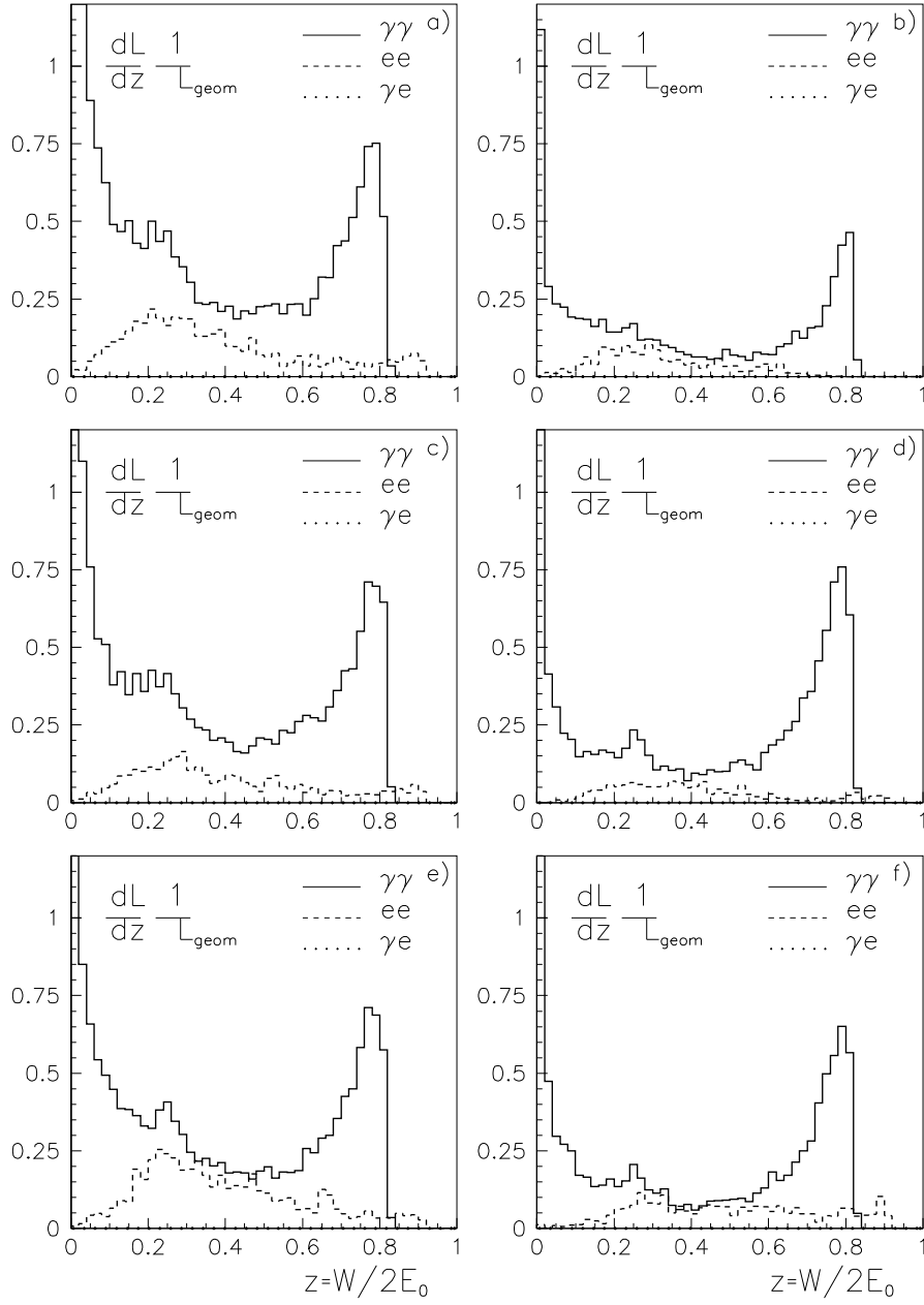
Figure 11: Spectral \gamma\gamma luminosity in the scheme with the vertical deflection for the beam parameters presented in Tables 2, 3 (Figs. 11a), b)... correspond to TESLA(1), TESLA(2)...). For additional comments see the text.
