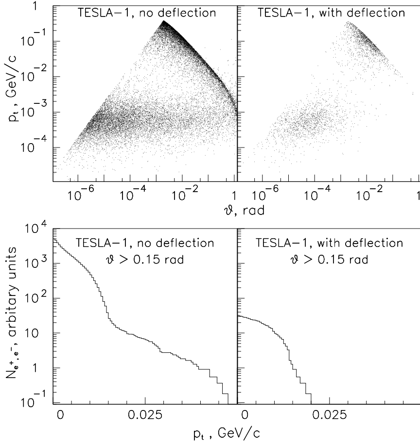
Figure 15: Upper figures: scatter plots of transverse momentum vs azimuthal angle, lower figures: p_{\perp} distribution of e^+e^- with \theta \geq 0.15 rad.
