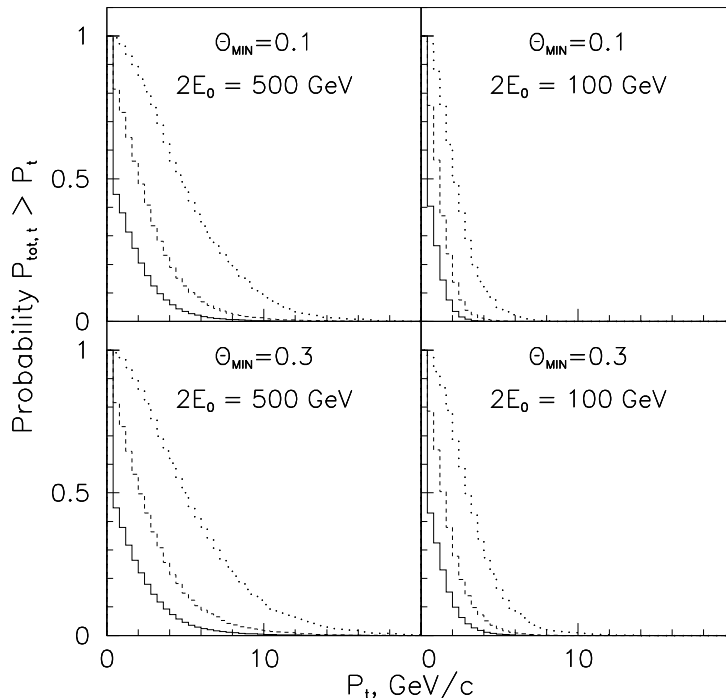
Figure 19: Probability to find an unbalanced transverse momentum above some p_t . Dotted, dashed and solid curves correspond to 7, 2, 0.7 \gamma\gamma \rightarrow hadrons events on the average per beam collision. The polar angle acceptance is \vartheta > 0.1 rad (upper plots) and \vartheta > 0.3 rad (lower plots). The collision energy is 500 GeV (left plots) and 100 GeV (right plots), photons have equal energies.
