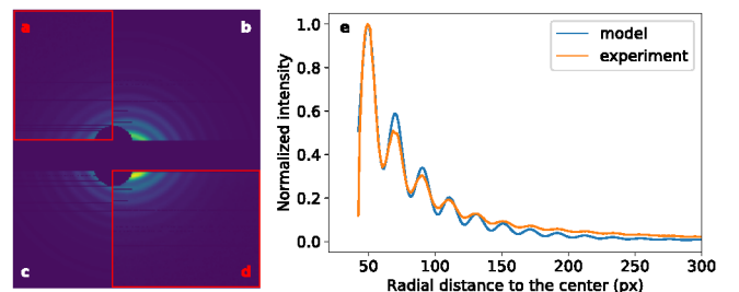
FIG. 2. Sum of 20964 diffraction patterns collected during 220 nm PS-particle injection; experimental data is provided in the red boxes (a, d) and compared to the fitted model. The left figure shows a section of the left half (a) and the right half (d) of the upper detector. The corresponding modeled sections (b, c) are flipped at the horizontal axis to allow for a detailed comparison. (e) Radial plot comparing the angularly integrated experimental and simulated data. Black stripes in the experimental data (a, d) are masked pixels and the exact same pixels were masked in the model in order to ensure comparability.
