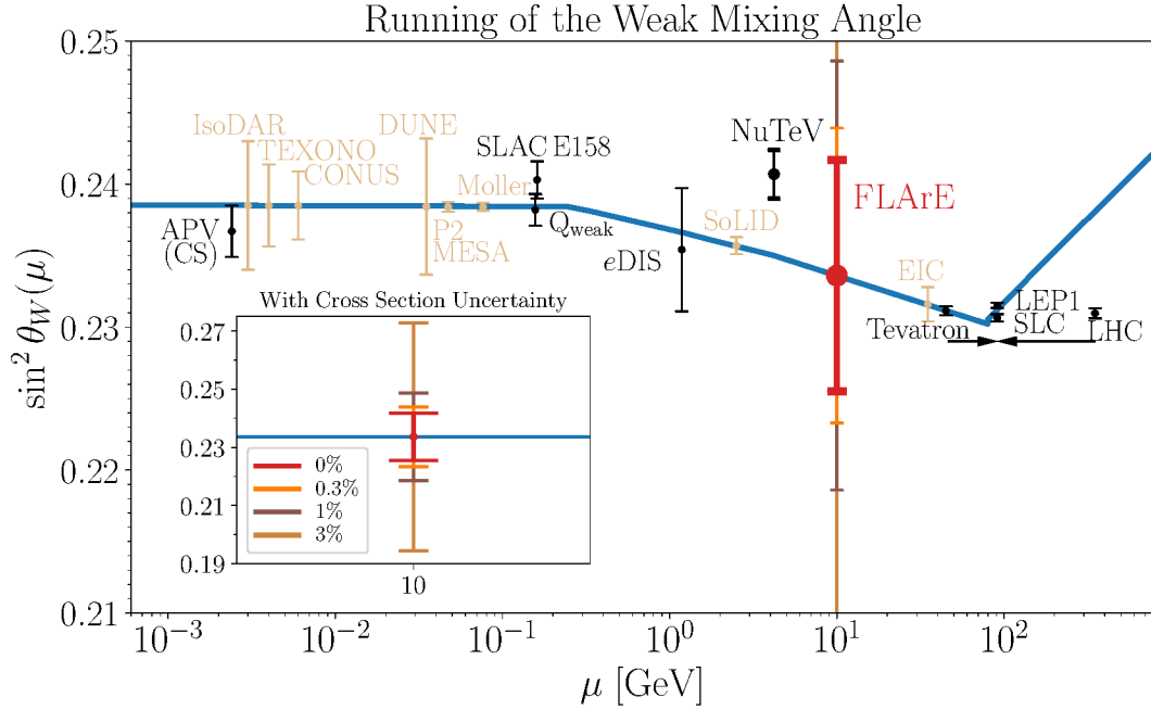
FIG. 3. Scale dependence of the weak mixing angle in the \overline{\text{MS}} scheme, \sin^2 \theta_W(\mu) , shown with the existing measurements (black), the expected sensitivity of FLArE at FPF (red), and other future experiments (beige). The blue line corresponds to the SM prediction for the running of \sin^2 \theta_W with scale \mu . For clarity, the Tevatron and LHC points are shifted horizontally on either side. Inset: We also show the sensitivity only at FLArE including a 3%, 1%, 0.3% and 0% systematic uncertainty on the neutrino-nucleus cross section.
