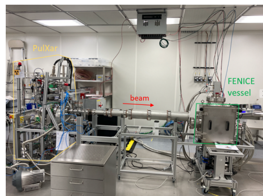
Fig. 2. Photograph of the experimental setup in the clean room (DET group, European XFEL). The 2 m long vacuum pipe connecting PulXar source and FENICE vessel (where the DEPFET ladder is instrumented) is visible in the centre.
