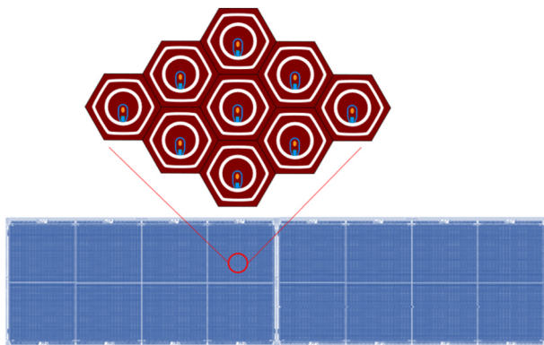
Fig. 1. Layout of the 128 x 512 pixel DEPFET ladder and of the hexagonal pixels.
