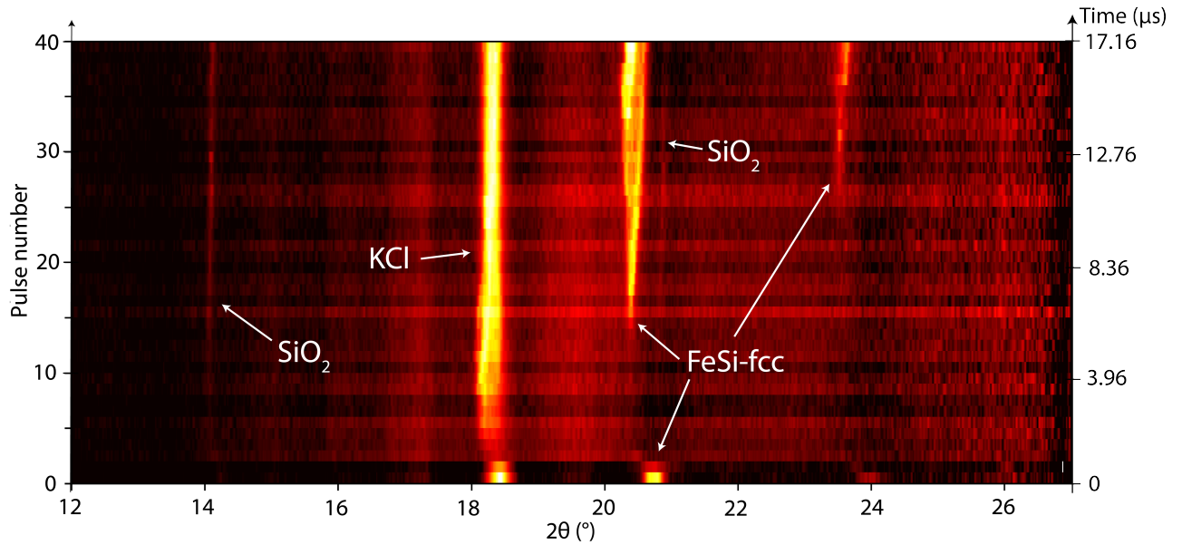
FIG. 3. Batch view of pulse train diffraction spectra series 23 . The pulse frequency was 2.257 MHz (time range span of 17.16 \mu s for 40 pulses). The moments where phases are first observed (spawn times) can be constrained by seeking the line apparition and checking for spots on the image plate. Observable phases are highlighted and designated. The KCl peak partly fades over the first pulses where the maximum fiber laser intensity is delivered to the sample, meaning that it is likely almost entirely molten inside the X-ray sampling zone. The first sample phase to crystallize upon cooling is \text{SiO}_2 . It is observed for the first time on the diffraction spectra at 2.2 \mu s (time zero corresponding to the first X-ray pulse). The FeSi-fcc peaks entirely disappear within the first 3 pulses before re-appearing at 5.72 \mu s for the left peak. Note that the second and fainter higher angle peaks of FeSi-fcc and \text{SiO}_2 appear later in time, likely due to signal degradation at higher angles and large crystal size.
