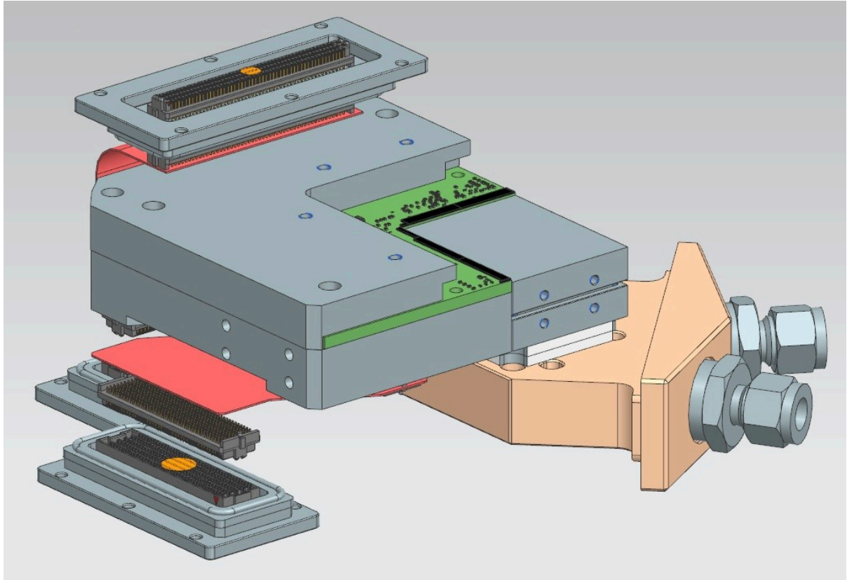
Figure 6. CAD rendering of the compact Percival 2M backside-illuminated CMOS camera.
