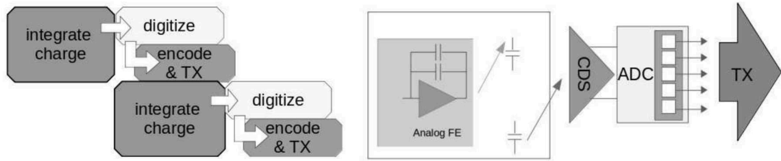
Figure 7: Pipelined approach adopted (left) and architecture of the readout ASIC (right). The Analogue frontend contains two memory circuits, while one is readout by the CDS, the other one is used to collect the next image.
