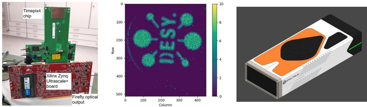
Figure 9 left: The TEMPUS system, comprising the custom carrier board, the Xilinx evaluation board, and the FMC+ Firefly board; middle: acquisition made in the time-stamping mode using a ^{55}\text{Fe} source and a DESY logo as target; right: future concept of a TEMPUS multi-chip system in collaboration with X-Spectrum.
