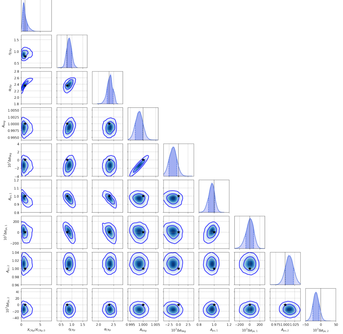
Figure 30. Example of posterior constraint on the full parameter space, as in Figure 14, but in the case of the pure hadronic model. Contours provide the 68% and 95% confidence interval. The black star shows the input model parameters.
