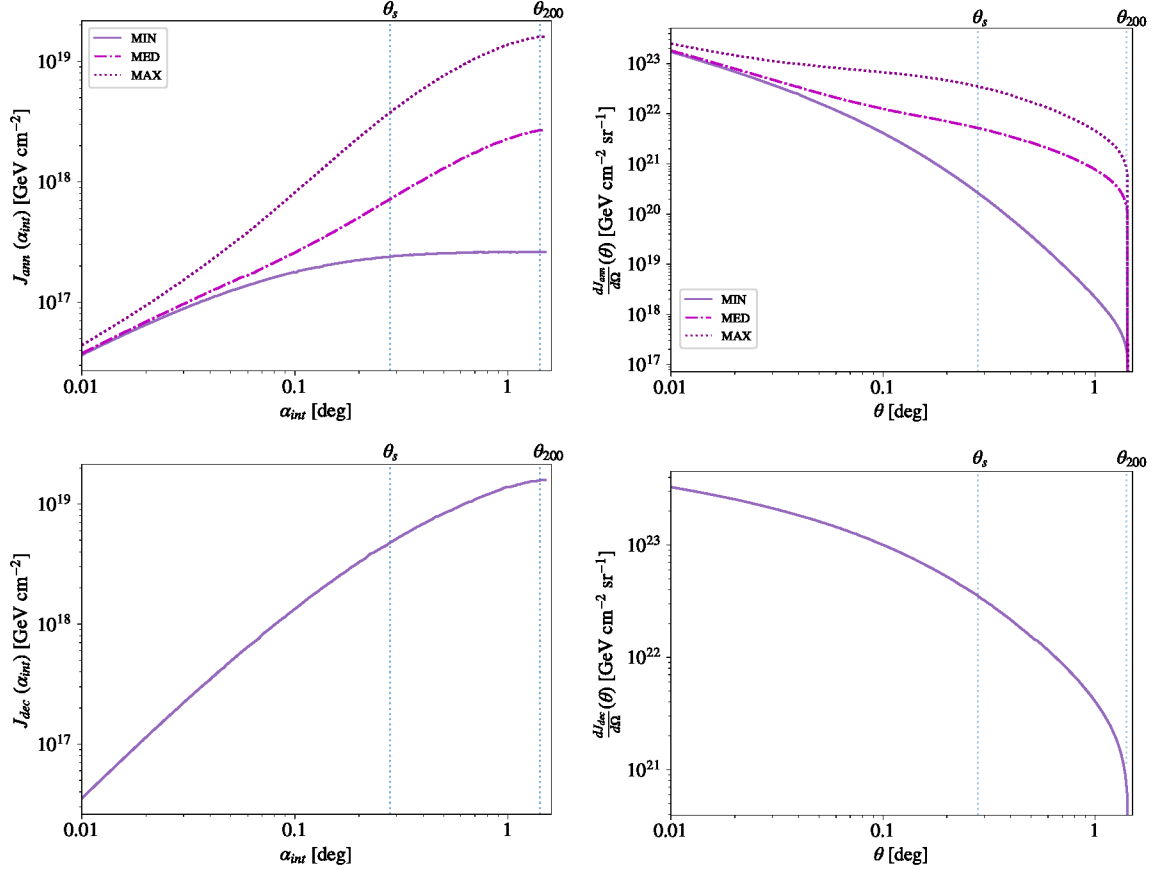
Figure 4. Integrated J-factors (Equation 3.3) versus the integration angle \alpha_{int} (left panels) and differential J-factors versus the radial angle \theta (right panels) for the annihilation scenario (top panels) and decay scenario (bottom panels) for the three substructure benchmark models correspondingly. In all the panels \theta_{200} and the projected angle of the scale radius, \theta_s , are shown as a measure of the containment of the emission and the extension of the cluster.
