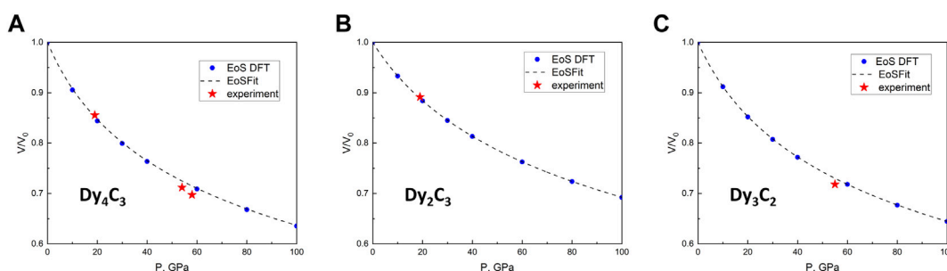
FIGURE 3 Pressure dependence of the relative volume for three Dy carbides. (A) \text{Dy}_4\text{C}_3 , (B) \text{Dy}_2\text{C}_3 and (C) \text{Dy}_3\text{C}_2 . The density functional theory (DFT)-calculated volumes for given pressures are shown by blue dots and dashed lines. Red stars indicate experimental data points.
