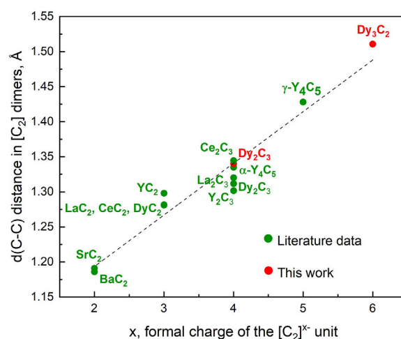
FIGURE 4 A correlation between the lengths of [\text{C}_2] dimers, d(\text{C}-\text{C}) , and their formal charges x in a number of binary metal-carbon compounds containing [\text{C}_2]^{x-} species. All data corresponds to ambient pressure. Literature data are from experiments [Atoji et al., 1958; Spedding et al., 1958; Atoji, 1967b; 1967a; Krupka et al., 1969; Adachi et al., 1976; Czekalla et al., 1997; Vohn et al., 2000; 1999; Yosida, 2002; Babizhetskyy et al., 2014; Aslandukova et al., 2021], except for \gamma\text{-Y}_4\text{C}_5 (Aslandukova et al., 2021) and for \text{Dy}_2\text{C}_3 and \text{Dy}_3\text{C}_2 (this work, DFT-computed structures fully relaxed at 1 bar).
