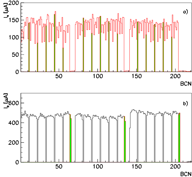
Fig. 2. The distributions of the electron (a) and proton (b) bunch currents (in \mu\text{A} ) in HERA. One histogram bin corresponds to a single Bunch Crossing Number (BCN) and shaded bins represent pilot bunches.
