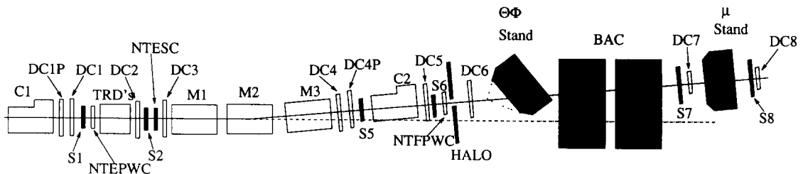
Fig. 4. Layout of experiment E790 apparatus in the Fermilab NT beam line.
