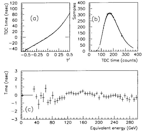
Fig. 10. (a) TDC counts versus T' . The fit is three parameter polynomial. (b) The pulse shape at the output of the shaper could be reconstructed by plotting the samples h_i versus the TDC counts in an asynchronous laser run. (c) Calculated time offsets (ns) versus equivalent energy (GeV).
