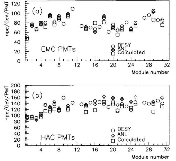
Fig. 9. Number of photoelectrons per GeV per PMT ( n_{pe} ) as a function of module. (a) EMC towers. (b) HAC towers.
