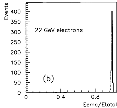
Fig. 6. (a) Typical TRD module. (b) E_{\text{EMC}}/E_{\text{total}} plot at 22 GeV. The fraction of entries in the peak around 1 shows the purity of the electron sample provided by the TRDs.
