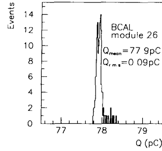
Fig. 8. Reconstructed charge in pC for a charge injector run for all channels of module 26. In this example, the fractional error on the charge reconstruction has an rms of about 0.1%.
