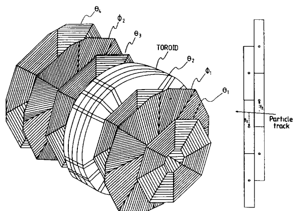
Fig. 1. (a) A schematic view of the forward muon spectrometer and (b) the cell structure of a double layer.
