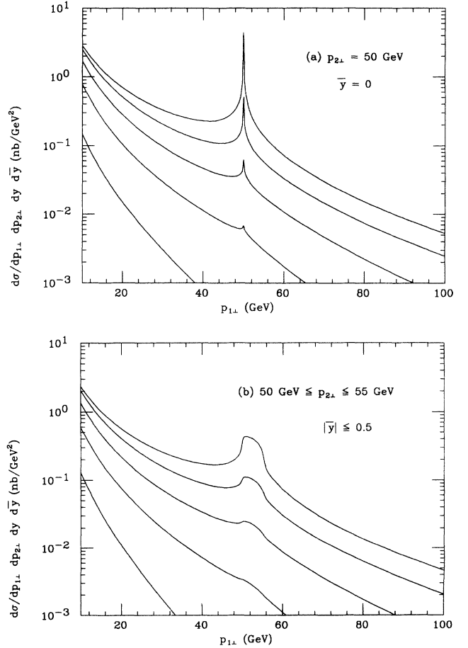
FIG. 5. p_{\perp} distribution of jet 1 with the jet 2 transverse momentum (a) fixed at 50 GeV, and (b) integrated from 50 GeV to 55 GeV. From top to bottom, the solid lines are the p_{\perp} distributions for the minijet-corrected cross section at |y| = 2, 3, 4, 5 , and 6. In (b) the rapidity boost \bar{y} is integrated over |\bar{y}| \leq 0.5 .
