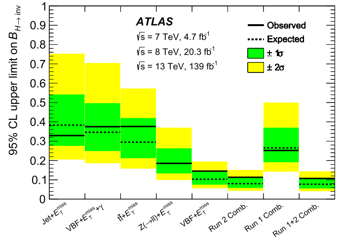
Fig. 3. The observed and expected upper limits on \mathcal{B}_{H \rightarrow \text{inv}} at 95% CL for the Run 2 analyses targeting the Jet + E_T^{\text{miss}} , VBF + E_T^{\text{miss}} + \gamma , t\bar{t} + E_T^{\text{miss}} , Z(\rightarrow \ell\ell) + E_T^{\text{miss}} , VBF + E_T^{\text{miss}} final states and their combination, the Run 1 combination and the full Run 1+2 result; the 1\sigma and 2\sigma contours of the expected limit distribution are also shown.
