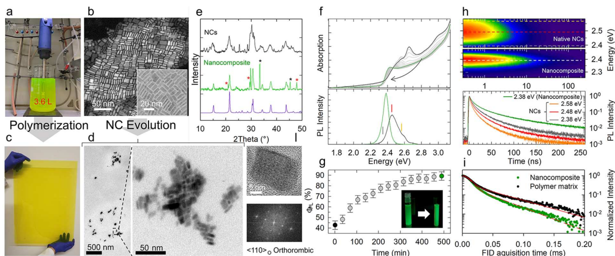
Figure 1. (a) Photograph of the turbo-emulsifier homogenized synthesis of 8 g of CsPbBr 3 NCs in a 5 L reactor. (b) STEM-HAADF image of the NC sample after washing. Inset: corresponding HRTEM image. (c) Photograph of a fabricated PMMA–PLMA nanocomposite with dimensions of 60 × 50 × 0.3 cm comprising CsPbBr 3 [NC] = 0.2 wt % under ambient illumination. (d) TEM micrographs of 70 nm thin nanocomposite section showing domains of CsPbBr 3 NCs in the polymeric matrix. (e) Powder X-ray diffraction patterns of the native NCs (top, black line) and of the NCs embedded in the nanocomposite displayed in panel c (middle, green line), together with the calculated PXRD pattern for orthorhombic CsPbBr 3 (bottom, purple line, ICSD 97851). The diffraction halo pattern associated with the polymeric host matrix in the PXRD of the nanocomposite was subtracted for clarity (Figure S6). The peaks denoted by star symbols are associated with minor crystalline impurities included in the nanocomposite (red stars, CsBr). (f) Optical absorption (top panel) and PL (bottom panel, excitation energy 3.1 eV) of 0.2 wt % dispersions of CsPbBr 3 NCs in LMA:MMA (20:80%vol) during the polymerization reaction (time evolution indicated by the black arrow). The initial spectra before the activation of the UV initiators and at the end of the process are highlighted in black and green, respectively. (g) Evolution of the PL quantum yield was observed during the polymerization process. The photographs of the liquid monomer mixture and the polymerized solid under UV illumination (3.4 eV) are reported as inset. (h) Contour plot of the spectrally resolved PL decay traces of the native NCs (top panel) and the final nanocomposite (middle panel) excited at 3.1 eV and (bottom panel) representative decay curves collected at the emission energies indicated by the dashed lines in the contour plots and the vertical bars in panel f. (i) 1 H NMR free induction decay (FID) at 333 K indicating faster relaxation for the nanocomposite (green dots, 0.2 wt %) with respect to the bare polymer matrix (black dots). The solid red lines are the fitting functions. (l) HRTEM image (top panel) and corresponding Fast Fourier Transform (FFT) pattern (bottom panel) of CsPbBr 3 NCs evolved in a solution of acrylate monomers.
