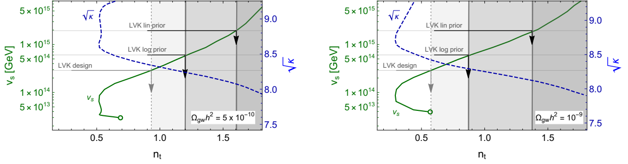
Figure 2: U(1) symmetry breaking scale v_s (solid green, left axis) and ratio \kappa^{1/2} between the monopole mass and the string tension (dashed blue, right axis) as a function of the predicted spectral tilt n_t of the SGWB, assuming an amplitude \Omega_{\text{gw}}^{\text{PTA}} h^2 \simeq 5 \cdot 10^{-10} (left) and \Omega_{\text{gw}}^{\text{PTA}} h^2 \simeq 10^{-9} (right) at f = 3 nHz. The grey region indicates values G\mu > 1.5 \cdot 10^{-8} ( G\mu > 1.6 \cdot 10^{-7} ) which are disfavoured by LVK for a logarithmic (linear) prior on the string tension [80].
