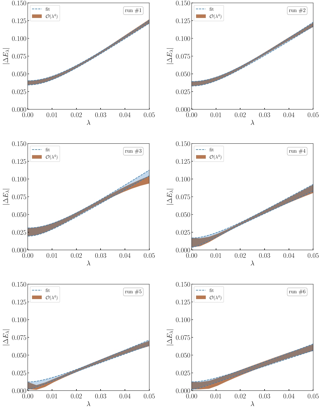
FIG. 10. The \lambda -dependence for runs #1 (top left), #2 (top right), #3 (center left), #4 (center right) #5 (bottom left) and #6 (bottom right) for \Delta E_\lambda . The numerical results at O(\lambda^4) are given as bands. The fits are given from using the square of Eq. (69) as further discussed in the text.
