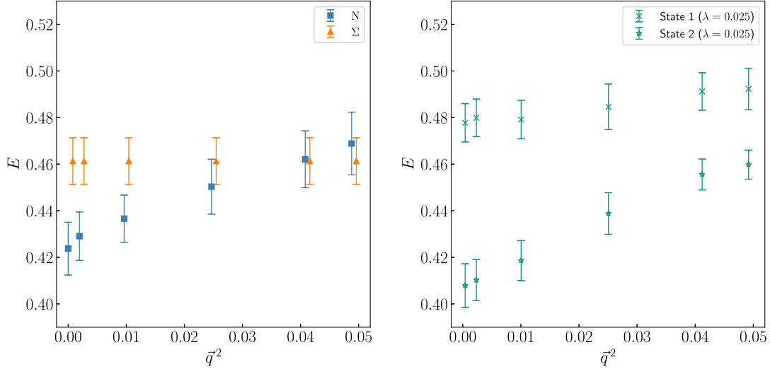
FIG. 11. LH panel: The noninteracting \Sigma mass (filled triangles) and N energy states (filled squares) as a function of \vec{q}^2 using the results of Table I. RH panel: The mixed states E_\lambda^{(-)} shown as crosses and E_\lambda^{(+)} shown as stars.
