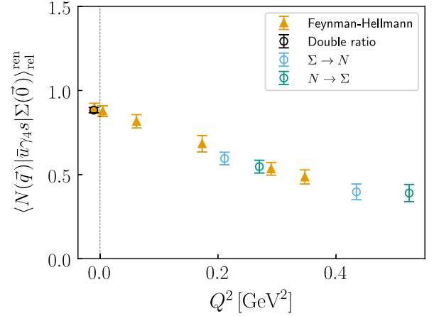
FIG. 13. Results for \langle N(\vec{q}) | \bar{u} \gamma_4 s | \Sigma(\vec{0}) \rangle_{\text{rel}}^{\text{ren}} versus Q^2 . Runs #1–#6 are given as (filled) triangles. We also make a comparison for this result with results using standard approaches to the computation. The (open) circles are results obtained from the three-point correlation function, Eq. (79) or the double ratio, Eq. (80).
