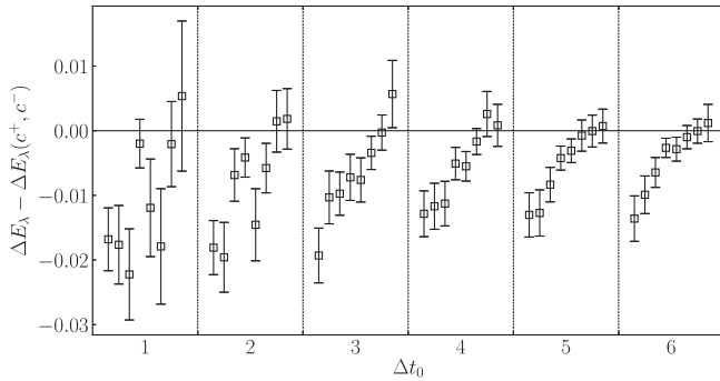
FIG. 7. The difference between two estimates of \Delta E_\lambda , one calculated from the eigenvalues of the GEVP and the other from a fit to the ratio of correlators in Eq. (74). The difference is shown as a function of both t_0 and \Delta t_0 . For each value of \Delta t_0 it is shown for the values t_0 = 1 - 8 , where the dashed lines separate the values of \Delta t_0 . These results are from run #5. The uncertainties are reduced for \Delta t_0 \geq 4 and they start agreeing with zero for t_0 \geq 6 .
