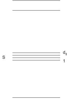
FIG. 1. A sketch of the energy levels. The set of quasidegenerate energy states are denoted by S , labeled from 1 to d_S . These states are well-separated from other states.
