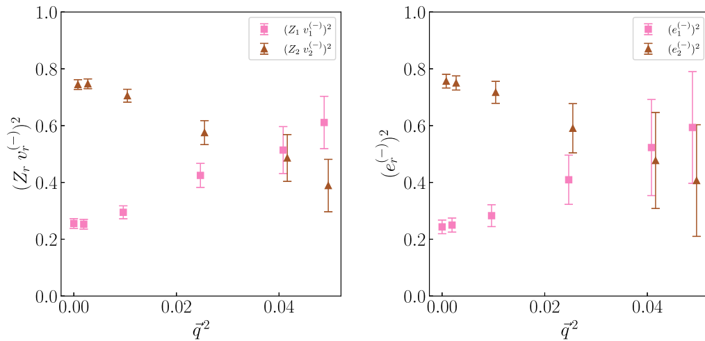
FIG. 9. LH panel: Normalized Z_r v_r^{(-)2} ( r = 1 squares, r = 2 triangles) against \vec{q}^2 . From Eq. (73) we see that these are equal to e_r^{(-)2} . RH panel: e_r^{(-)2} , ( r = 1 squares, r = 2 triangles) from Eq. (55) against momentum \vec{q}^2 . Both plots are for \lambda = 0.025 .
