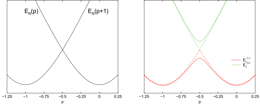
FIG. 2. LH panel: A sketch of the (unperturbed) energy states E_N(p) , E_N(p+q) versus p in one dimension for fixed q using units where q = 1 . Using these units there is a degeneracy at p = -1/2 . RH panel: An equivalent sketch of the perturbed energy states, E^{(\pm)} based on Eq. (53). The dashed lines are the free case. The sketch shows the avoided energy levels.
