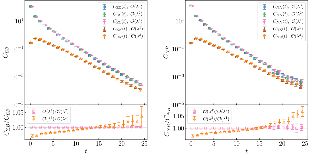
FIG. 5. LH panel: The C_{\lambda\Sigma\Sigma} correlation functions at O(1) , O(\lambda^2) and O(\lambda^4) , (squares, circles and stars, respectively) and C_{\lambda\Sigma N} correlation functions at O(\lambda) and O(\lambda^3) (upper triangles and lower triangles, respectively) at \lambda = 0.025 against t for t_0 = 6 and \Delta t_0 = 4 . The lower subplot shows the ratio of correlation functions C_{\lambda\Sigma B} ( B = \Sigma , squares and B = N , triangles) between the two highest orders of \lambda available. RH panel: Similarly for C_{\lambda NN} and C_{\lambda N\Sigma} . The points are slightly offset for visibility. Both results are for run #5 where # denotes the run number.
