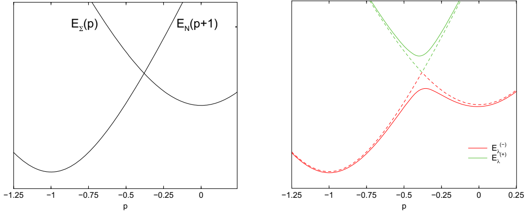
FIG. 3. LH panel: A sketch of the (unperturbed) energy states E_\Sigma(p) , E_N(p+q) versus p in one dimension for fixed q using units where q = 1 . RH panel: An equivalent sketch of the perturbed energy states, E^\pm . The dashed lines are the free case. The sketch shows the avoided energy levels.
