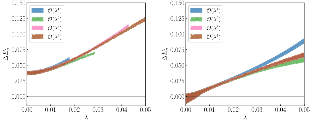
FIG. 8. LH panel: The \lambda -dependence for run #1 for \Delta E_\lambda . The numerical results for each order in \lambda ( O(\lambda) , O(\lambda^2) , O(\lambda^3) and O(\lambda^4) ) are given as bands. RH panel: Similarly for run #5.
