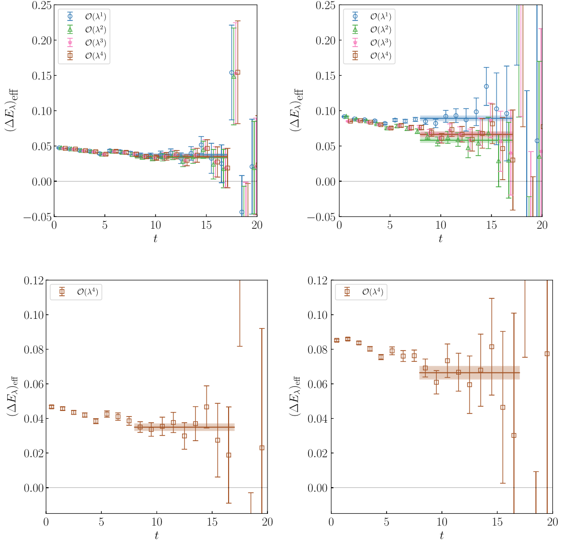
FIG. 6. Upper LH panel: (\Delta E_\lambda)_{\text{eff}} versus t for \lambda = 0.025 at O(\lambda) (circles), O(\lambda^2) (triangles), O(\lambda^3) (stars), O(\lambda^4) (squares) for run #5. Upper RH panel: Similarly for \lambda = 0.05 . The points are slightly offset for visibility. Also shown is the fit interval used and fit using Eq. (74). Lower LH plot: An expanded plot of the upper LH plot at O(\lambda^4) (squares). Lower RH plot: Similarly for the upper RH plot.
