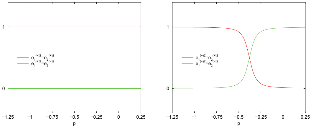
FIG. 4. Left panel: The free case where we have plotted e_1^{(-)2} and e_2^{(-)2} against p , again taking units where q = 1 . Right panel: The interacting case showing the change of state.
