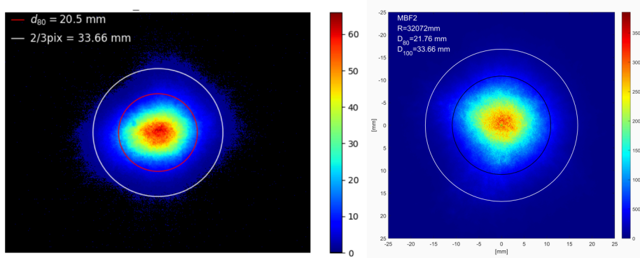
Figure 5: PSF at best focus of the MBF 1 mirror (mosaic of 4 elements) measured using the INP PAS testing setup (left, red circle) and the MBF 2 mirror (mosaic of 7 elements) measured with the JLO test bench (right, blue circle). White circles show d_{100} = 33.66 mm containment radius.
