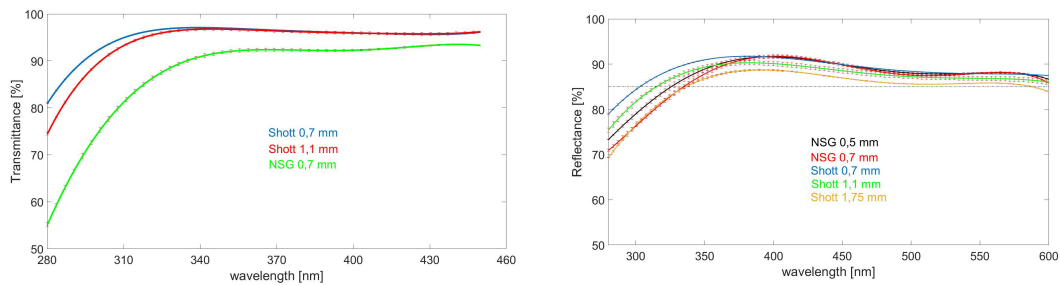
Figure 1: Comparison of spectral transmittance (left) and reflectance (right) in the UV-VIS waveband of thin glass samples of SCHOTT Borofloat® 33 and NSG glanova™ glass. The samples are coated with Al on their back surfaces.
