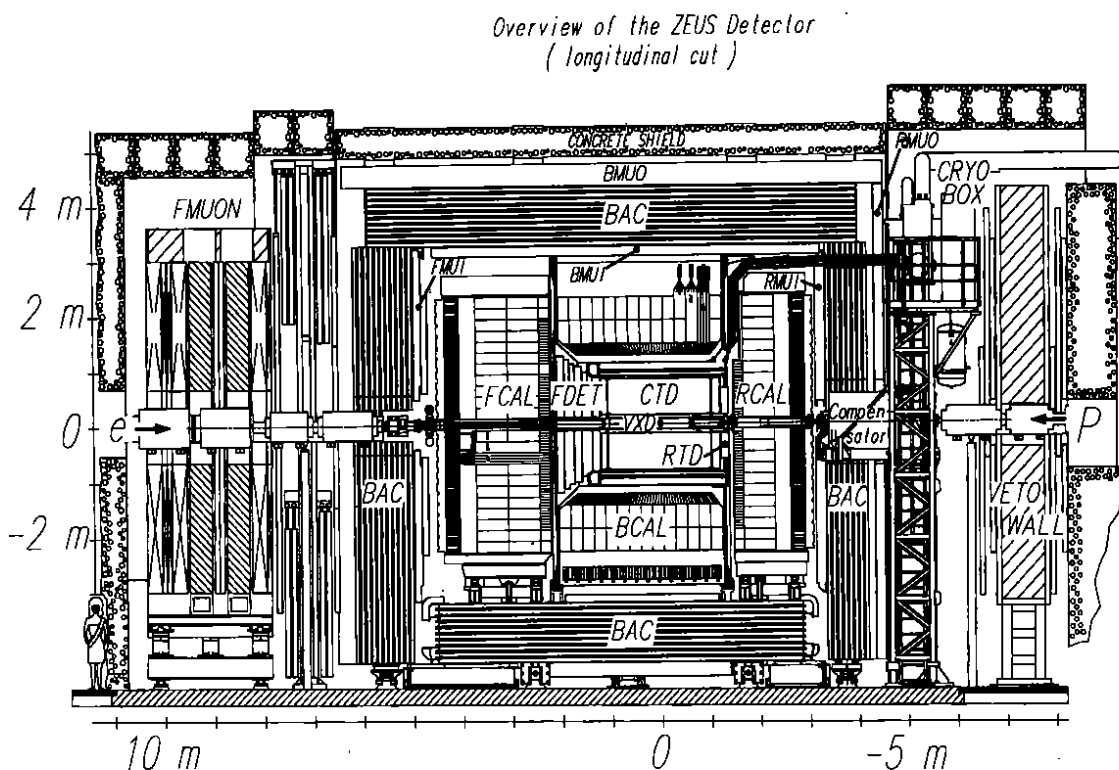
Figure 1: A side view of ZEUS.
