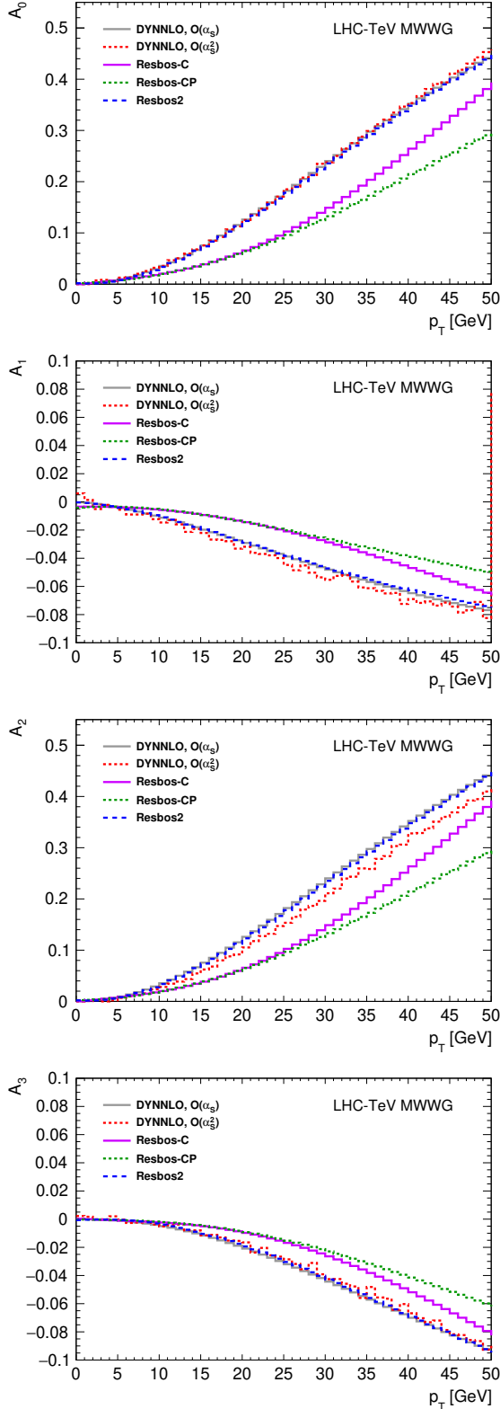
Fig. 6: A_0 to A_3 as a function of p_T^W extracted from RESBOS-C, RESBOS-CP, RESBOS2, DYNLO at \mathcal{O}(\alpha_s) , and DYNLO at \mathcal{O}(\alpha_s^2) in p\bar{p} collisions at 1.96 TeV. The CTEQ6M PDF set is used for all generators except RESBOS-CP, for which CTEQ6.6 is used. The RESBOS-C and RESBOS2 calculations are at \mathcal{O}(\alpha_s) in QCD, and RESBOS-CP is at \mathcal{O}(\alpha_s^2) . The difference between DYNLO at \mathcal{O}(\alpha_s) and \mathcal{O}(\alpha_s^2) has an \mathcal{O}(1 \text{ MeV}) effect on \delta m_W^{\text{pol}} .
