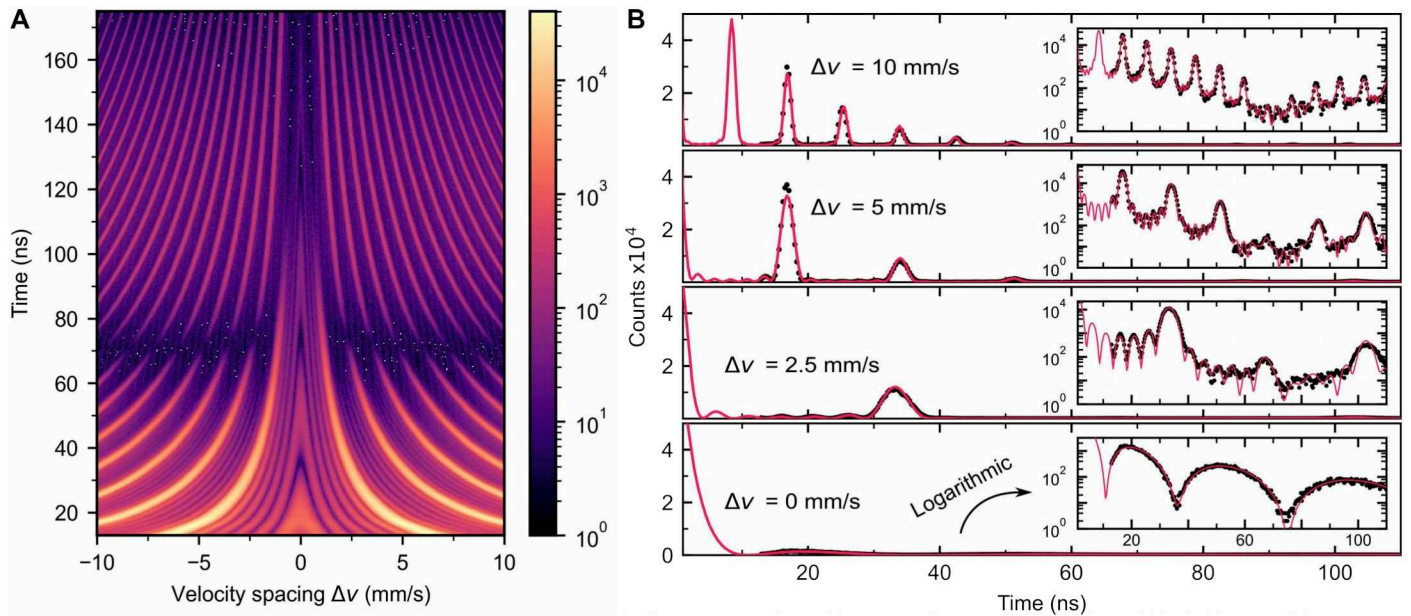
Fig. 2. Single photon decay from nuclear frequency comb. (A) Time-velocity histogram of the single photon decay of a nuclear exciton spectrally prepared in a frequency comb consisting of seven teeth, equally spaced over a Doppler detuning range extending from -10 mm/s to 10 mm/s ( \approx 480 neV). The color map displays the number of detected photons on a logarithmic scale. (B) Decay histogram for four selected velocity spacings from (A) in linear and logarithmic scales. The patterns are simulated using the software package Nexus (red).
