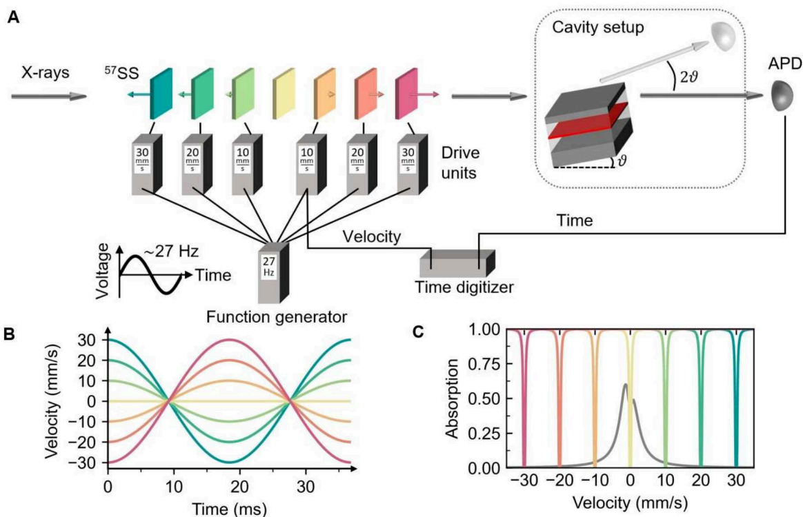
Fig. 1. Experimental setup. (A) Six isotopically enriched 3.2 \mu\text{m} thick ^{57}\text{Fe} stainless steel foils ( ^{57}\text{Fe}_{0.55}\text{Cr}_{0.25}\text{Ni}_{0.2} %wt.; ^{57}\text{SS} ) are mounted on six Mössbauer transducers (not shown), each individually driven by a drive unit. A seventh ^{57}\text{Fe} foil is kept at rest. Each drive unit amplifies the AC voltage generated by a single function generator differently, such that the foils move with maximum velocities of 30 mm/s, 20 mm/s, 10 mm/s, -10 mm/s, -20 mm/s and -30 mm/s. The negative sign indicates a 180^\circ motional phase shift realized by flipping the respective transducer. The nuclear resonance is excited by X-ray pulses from the synchrotron. The photon detection time and the instantaneous velocity of one Mössbauer transducer are simultaneously recorded using a multiple-event time digitizer. The cavity is mounted optionally (sequence of cavity and foils is irrelevant, see Supplemental Materials). (B) Velocity profile of each foil, following the 27 Hz AC driving voltage. (C) Combined nuclear resonant absorption spectrum of the foils driven at maximum velocity, resulting in a frequency comb with a velocity spacing of 10 mm/s ( = 480 neV). The spectrum of the single photon wave packet emitted by the cavity is plotted in the background (arb. u.).
