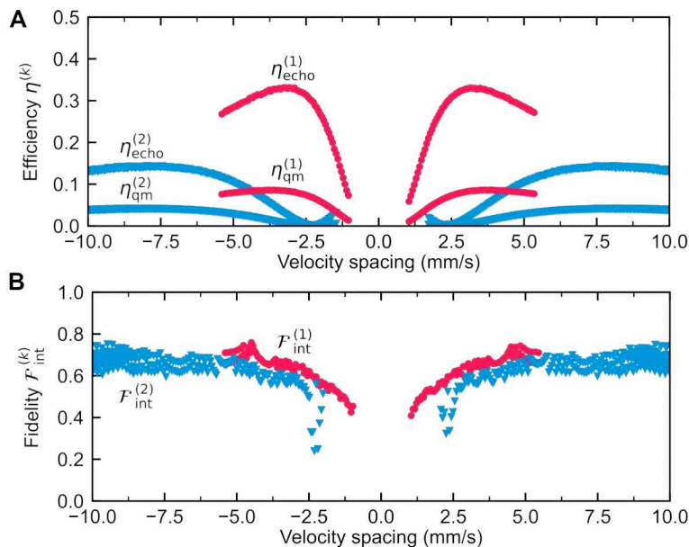
Fig. 4. Quantum memory parameters. Derived echo efficiency \eta_{\text{echo}}^{(k)} , quantum memory efficiency \eta_{\text{qm}}^{(k)} (A) and intensity fidelity F_{\int \delta^{(k)} \delta} (B) for the k -th echo [ k=1 (red) or k=2 (blue)] of the cavity-frequency comb setup as a function of the velocity spacing. For echoes appearing early, < 13 ns (detection dead time), or late, at > 100 ns (low intensity), no meaningful values of efficiency and fidelity could be derived.
