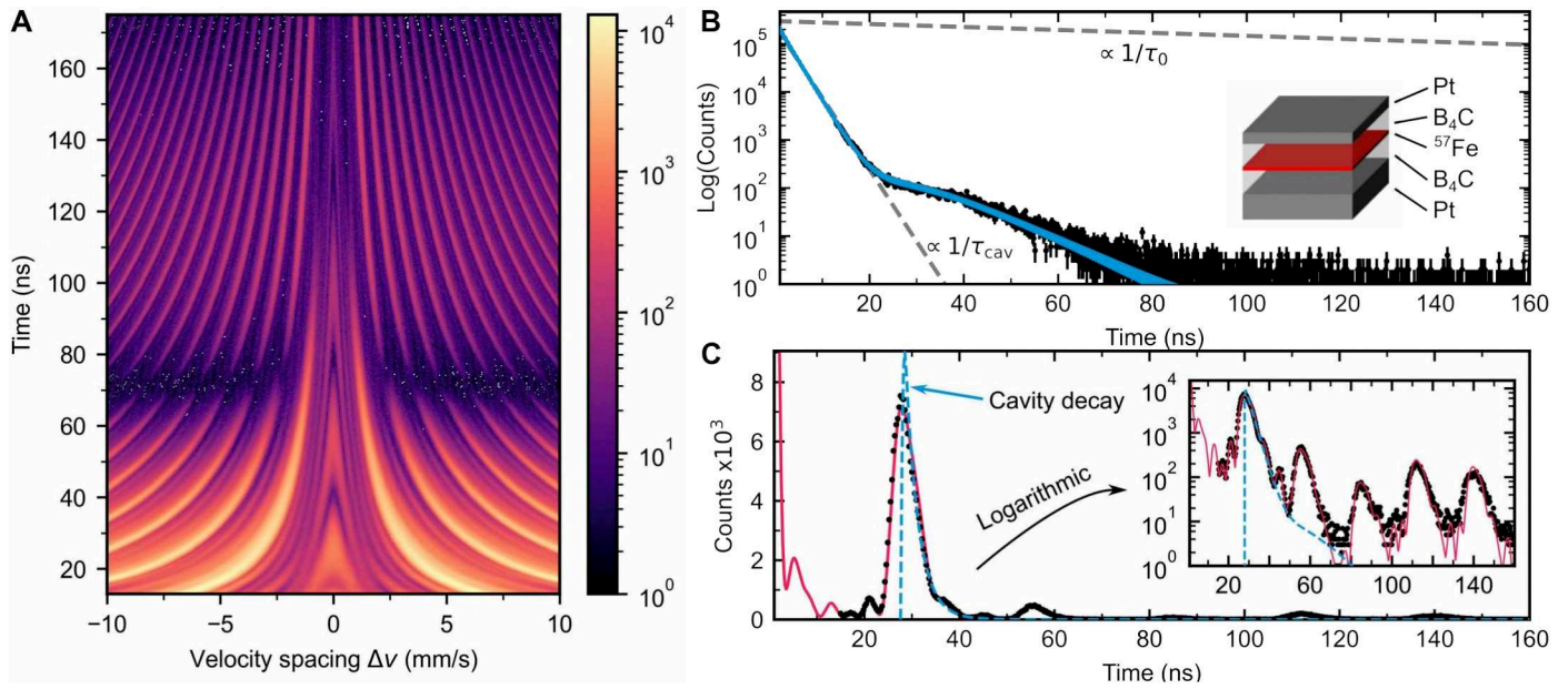
Fig. 3. Quantum memory data. (A) Time-velocity histogram of the same frequency comb as shown in Fig. 2, in combination with a thin film cavity excited in its first waveguide mode at an incident angle of 0.1505^\circ . (B) Measured (black) and fitted (blue) decay histograms of the thin film cavity alone, excited in its first waveguide mode. The initial strong speed-up in the cavity decay corresponds to an exponential decay [ \propto \exp(-t/\tau_{cav}) ], with \tau_{cav} = 2.9(2) ns, in comparison to the natural exponential decay of the excited ^{57}\text{Fe} state with \tau_0 = 141 ns. The inset shows the layer structure of the cavity consisting of: Pt (2.3 nm)/ \text{B}_4\text{C} (13.1 nm)/ ^{57}\text{Fe} (1.1 nm)/ \text{B}_4\text{C} (12.8 nm)/ Pt (15.0 nm)/ \text{Al}_2\text{O}_3 (substrate; not shown). (C) Extracted decay histogram from (A) at the velocity spacing of 3.1 mm/s ( \approx 240 neV) with measurement (black) and fit (red) in linear and logarithmic scales. The derived cavity decay from (B) is overlaid (blue) at the first echo, showing the matching decay of the echo and the cavity intensities. More decay histograms for different velocity spacings are depicted in the Supplementary Materials.
