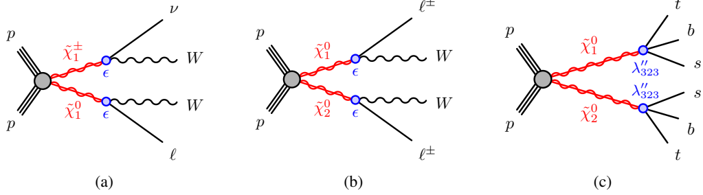
Figure 2: Diagrams of the targeted RPV models. Diagrams (a) and (b) serve as examples, since inclusive bRPV production is considered. The UDD RPV scenario with BNV terms in diagram (c) is a simplified model.
