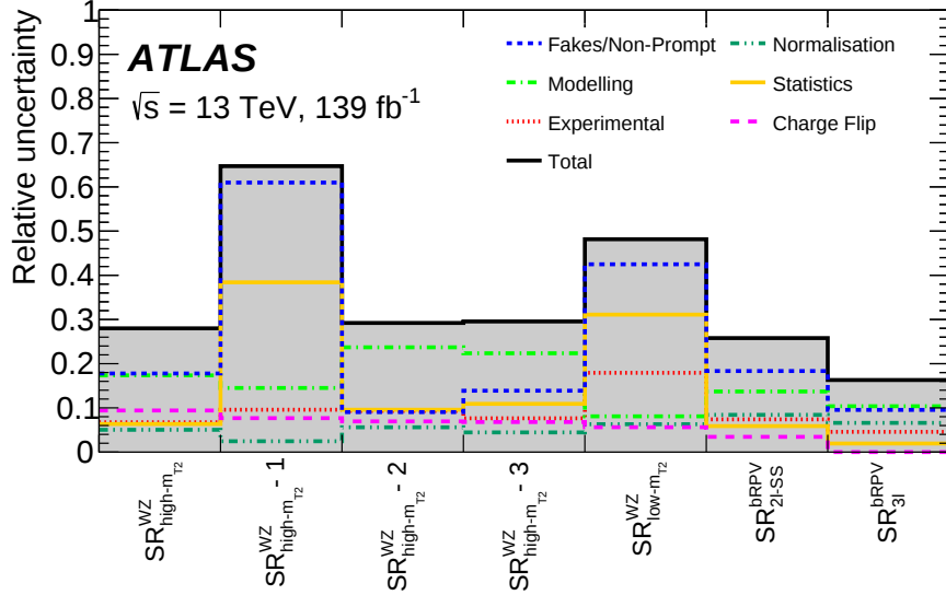
Figure 7: Breakdown of the total systematic uncertainty in the background prediction for each of the SRs of the WZ and bRPV models. Total and individual uncertainties for different source categories are shown. The individual components can be correlated and therefore do not necessarily add up in quadrature to the total systematic uncertainty.
