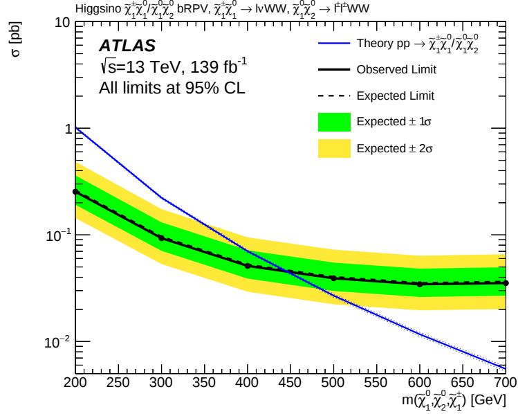
Figure 14: Observed (black solid line) and expected (black dashed line) 95% CL exclusion limits as a function of higgsino \tilde{\chi}_1^0/\tilde{\chi}_2^0/\tilde{\chi}_1^\pm mass in the bilinear RPV model. The green (yellow) contours of the band around the expected limit are the \pm 1\sigma ( \pm 2\sigma ) variations including all uncertainties. The prediction for the theoretical production cross section is also shown (blue solid line) with its uncertainty (blue dotted lines).
