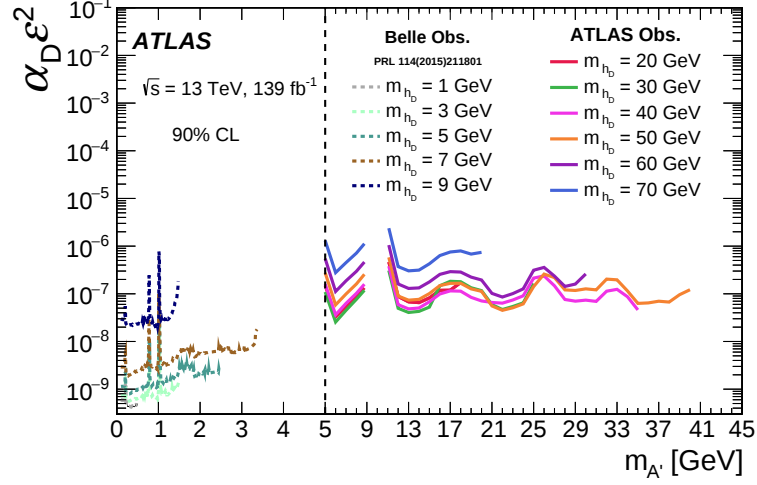
Figure 4: Observed 90% CL upper limits on \alpha_D \epsilon^2 , as a function of m_{A'} with different dark Higgs boson masses, from this search (solid curves) compared with the results from Belle [15] (dashed curves).
