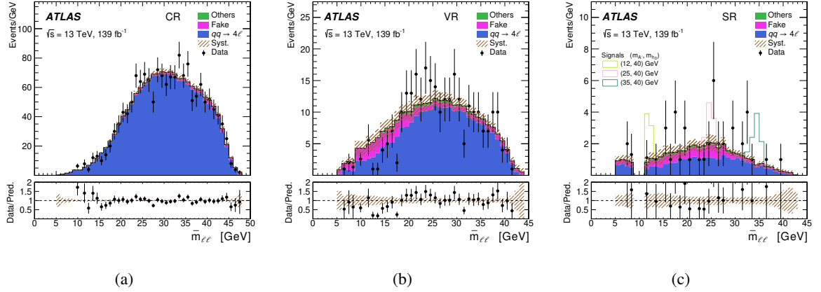
Figure 2: The \bar{m}_{\ell\ell} distribution in the (a) CR, (b) VR and (c) SR for the data and post-fit background contributions. The error bands include experimental and theoretical systematic uncertainties as constrained by a background-only fit. The contributions from the production of qq \rightarrow 4\ell events are scaled by a normalization factor 0.95, from the simultaneous fit in the SR and CR. The “Others” category combines gg \rightarrow ZZ , Higgs, VVV and ttZ background contributions. The “Fake” background represents the contribution from non-prompt leptons. Three representative signal distributions are overlaid in the SR, assuming m_{h_D} = 40 GeV and different values of m_{A'} . The cross-sections for these benchmark points are calculated with \alpha_D = 0.1 and \varepsilon = 10^{-3} .
