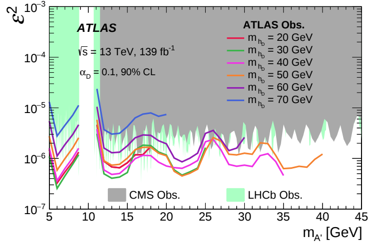
Figure 5: Observed 90% CL upper limits on \epsilon^2 , assuming of \alpha_D = 0.1 , as a function of m_{A'} with different dark Higgs boson masses ranging from 20 GeV to 70 GeV. The parameter space excluded by LHCb [12] (CMS [74]) is covered by the green (gray) shaded regions.
