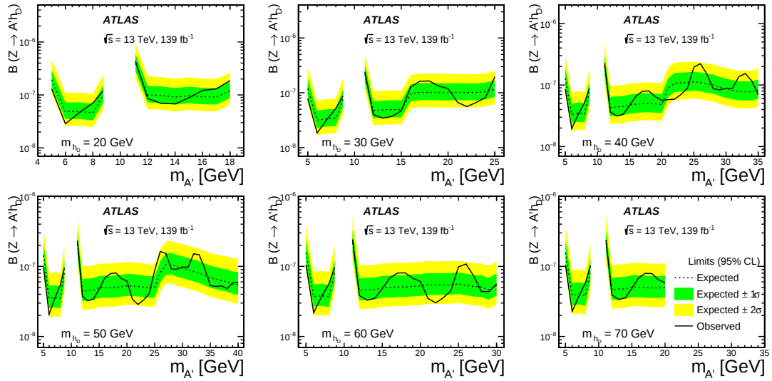
Figure 6: Observed and expected upper limits at 95% CL on the branching fraction \mathcal{B}(Z \rightarrow A' h_D) as a function of m_{A'} , from top left to bottom right corresponding to the dark Higgs boson mass of 20 GeV, 30 GeV, 40 GeV, 50 GeV, 60 GeV, and 70 GeV, respectively. The green (inner) and yellow (outer) bands represent the \pm 1\sigma and \pm 2\sigma uncertainty in the expected limits.
