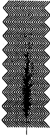
Figure 24 : A 40 GeV electron showering in a lead liquid argon accordion structure. The lead absorber plates run at \pm 45^\circ to the particle direction thus avoiding channelling. Preamplifiers are located at the front and at the back of the calorimeter, minimizing the connection capacitances.
