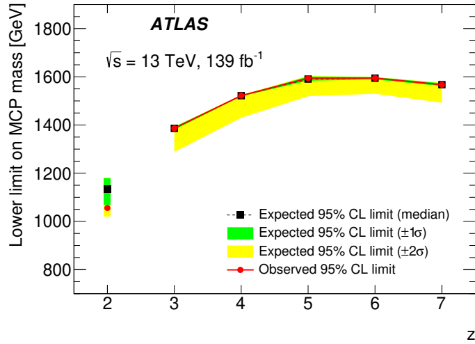
Figure 9: Observed and expected 95% CL lower mass limits of MCPs versus charge. The separation of limits between z = 2 and z = 3 is due to different selections used to identify MCPs with the respective charges.
