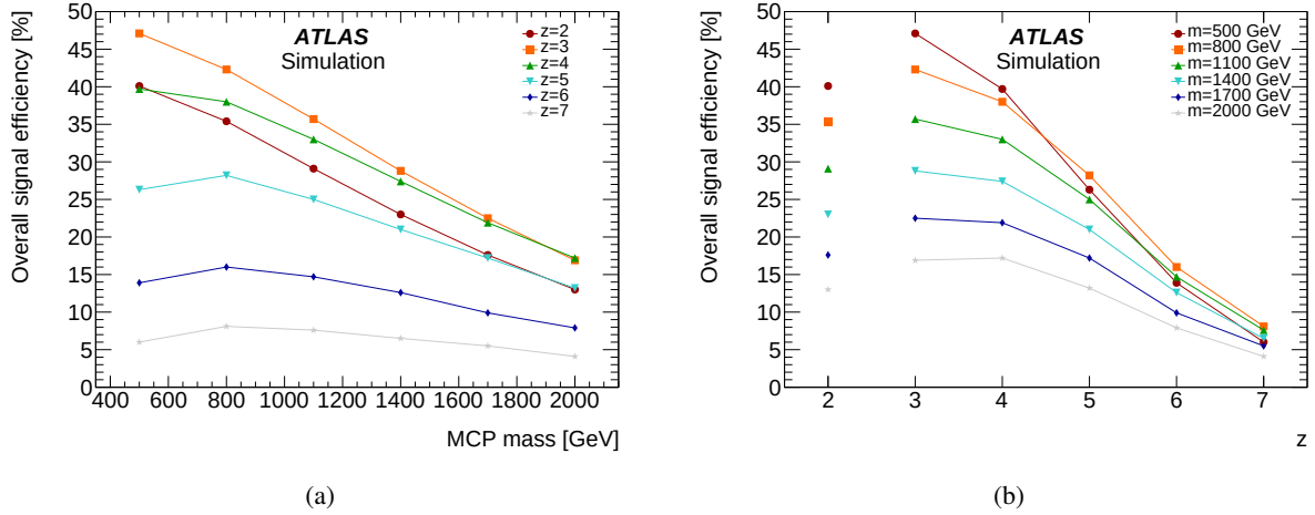
Figure 5: The signal efficiencies for spin- 1/2 MCPs with different charges and masses for the DY+PF production mode versus (a) their mass and (b) their charge. Efficiency values for z = 2 in (b) are separated from the rest of the plot to reflect different signal selections used in the two search categories.
