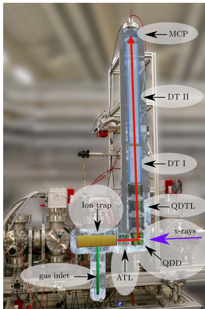
Figure 1. Overview of the ion trap at the PIPE setup. The soft X-ray beam enters from the right. The ions leave the ion trap to the right via the after-trap lens (ATL) system. The extracted ions are deflected upward by the electrostatic quadrupole deflector (QDD) and focused with a quadrupole-triplet lens (QDTL) into the drift tubes DT I and DT II. The ions are detected using a Chevron microchannel-plate (MCP) stack. The red line indicates the ions’ flight path.
