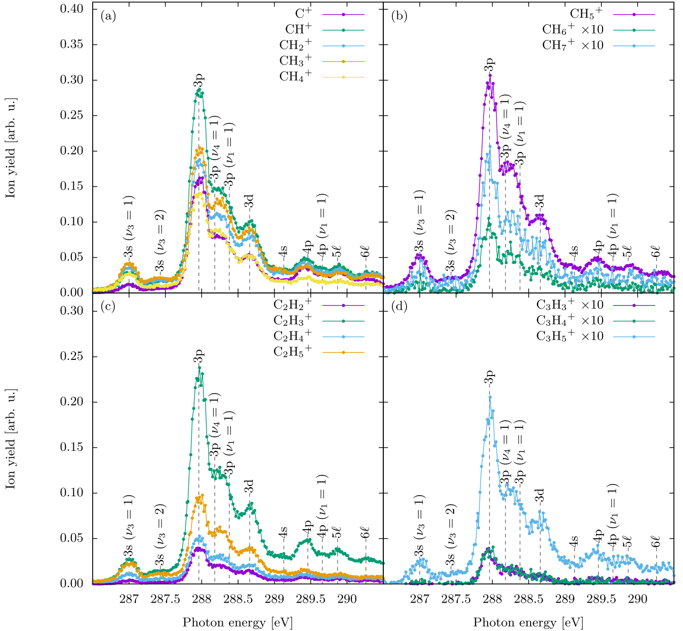
Figure 4. (a) Measured relative cross sections (product-ion yields) for photoionization and fragmentation of methane at the C 1s edge. Every photoabsorption product in this trap experiment can react with neutral methane. (b) Photon-energy dependencies of hydrogen-addition reaction channels. Note that the \text{CH}_6^+ and \text{CH}_7^+ yields have been multiplied by a factor of 10. (c) Photon-energy dependencies of dimerization channels of methane. Channels shown in (b) and (c) can only occur when ionic photoabsorption products, which are shown in (a), collide with at least one neutral methane molecule while stored in the trap. (d) Photon-energy dependencies of the trimerization of methane. These reaction products can only be formed by at least two methane-addition steps. Note that the yields in panel (d) have been multiplied by a factor of 10.
