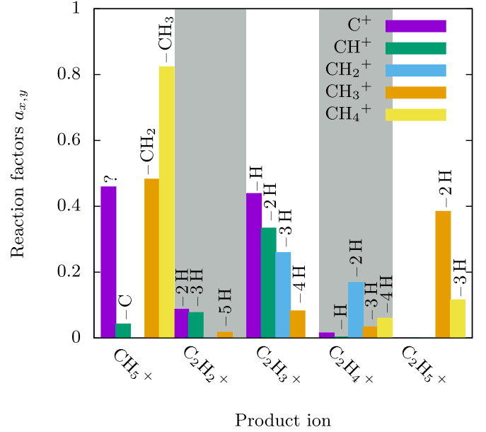
Figure 6. Reaction factors a_{x,y} as obtained from the linear combination model (Equations (4) and (5)). The neutral elimination products resulting from the ion–methane reaction are written on the respective bars. Since for \text{CH}_5^+ the differences between the resonances are very small, the algorithm assumes a mixture of different ions. This is a weak point of the linear combination model. \text{CH}_5^+ cannot originate from a reaction between \text{C}^+ and a methane molecule. For this reason we put a question mark on the respective bar (for further discussion see text). The uncertainties of the individual contributions represented by the bars are around 10%.
