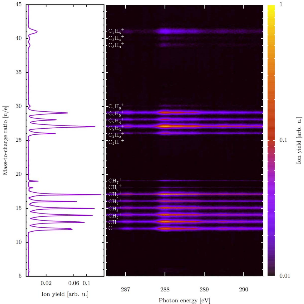
Figure 2. NEXAFS (near edge X-ray absorption fine structure) ion time-of-flight map of methane at the C 1s edge measured after a certain trapping time of 3 ms. In addition to the primary \text{CH}_x^+ photofragment series, secondary heavier molecular ions are clearly observed which can only be the products of additional reactions of primary fragments with neutral methane molecules. These products are identified as \text{C}_2\text{H}_x^+ and \text{C}_3\text{H}_x^+ ions which incorporate two or three carbon atoms.
