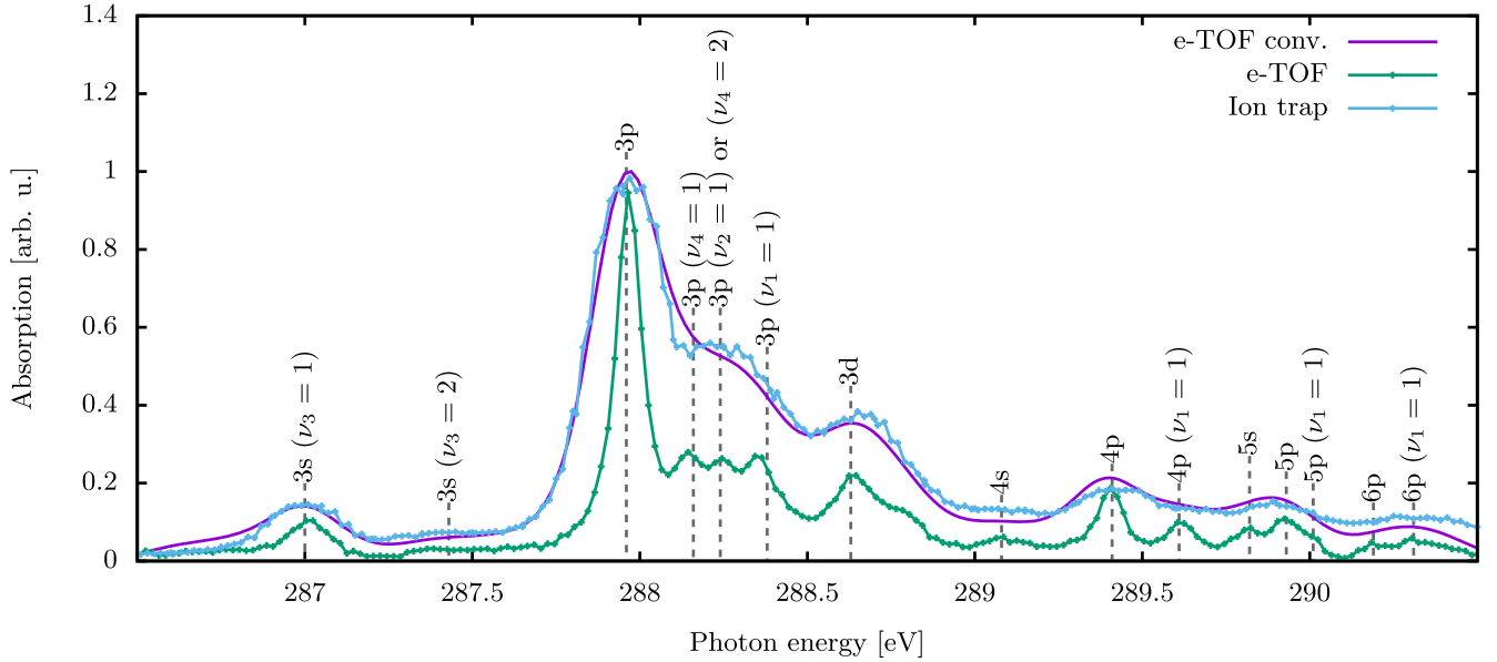
Figure 3. The photoabsorption spectrum of methane measured with the ion trap compared to an electron-yield spectrum obtained with an electron time-of-flight (e-TOF) spectrometer. The latter spectrum was recorded by 16 identical time-of-flight electron detectors, which are housed in the diagnostic unit of the soft X-ray beamline P04 (Buck et al. 2019). For comparison of the e-TOF result with the lower-resolution ion-trap data, the energy resolution was adapted to the experimental resolution by convolution with a 0.2 eV FWHM Gaussian function.
