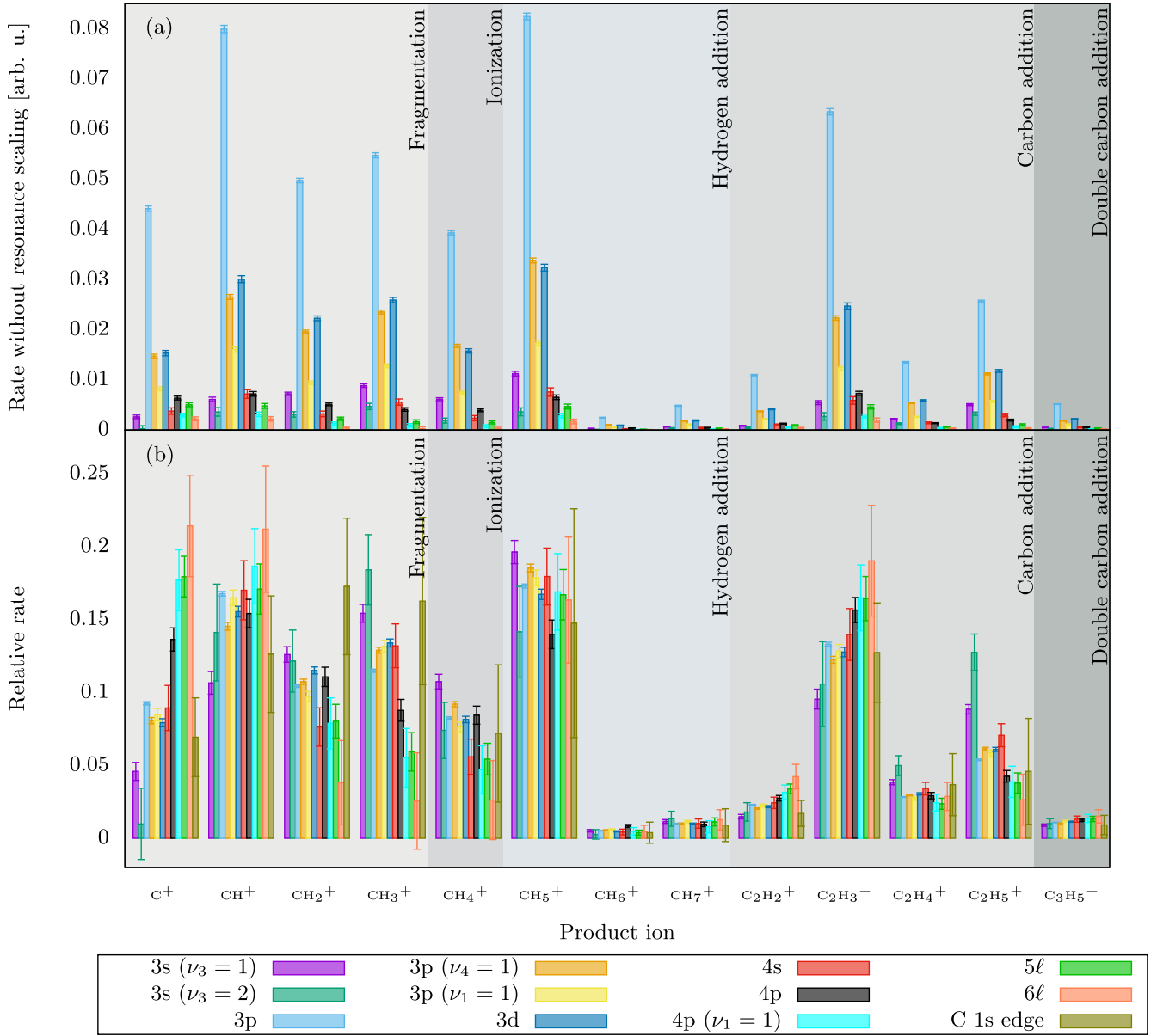
Figure 5. The areas of the individual resonances determined from the Voigt fits in relative units are shown in panel (a). In addition to the simple methane ionization channels, the fragmentation channels and the reaction channels are also shown. To enable a comparison between the resonances, the composition of the channels is shown in panel (b). In order to obtain the composition for each resonance, the sum of the different product ions was set to one for each resonance.
