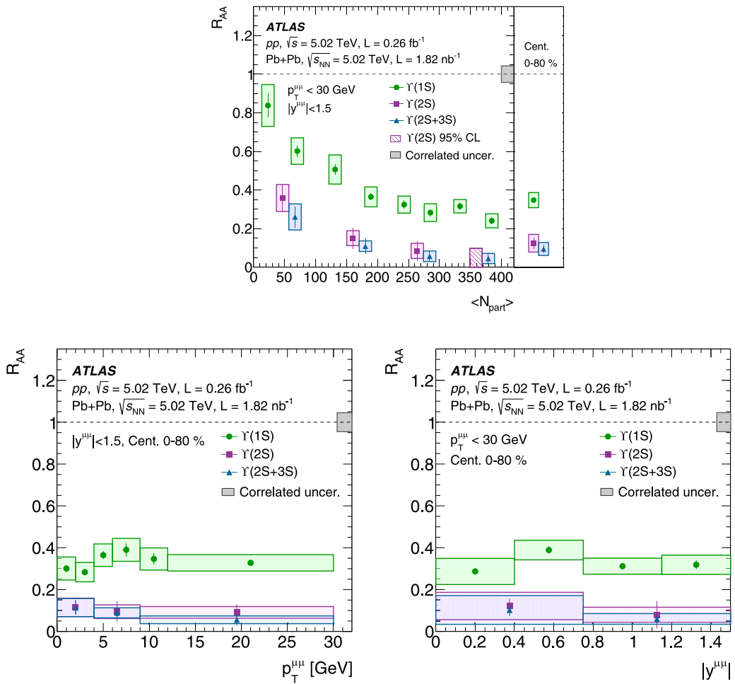
FIG. 3. The nuclear modification factor R_{AA} of \Upsilon(1S) , \Upsilon(2S) , and \Upsilon(2S + 3S) as functions of centrality (top), p_T^{\mu} (bottom left), and |y^{\mu}| (bottom right) at 5.02 TeV. Error bars indicate the statistical uncertainties and boxes represent the systematic uncertainties. The gray boxes around R_{AA} = 1 correspond to the global systematic uncertainty. The right panel of the top plot shows the R_{AA} results integrated over centrality.
