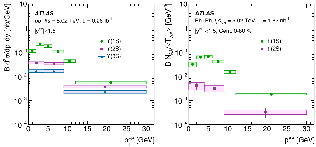
FIG. 2. Production cross sections of \Upsilon(1S) , \Upsilon(2S) , and \Upsilon(3S) mesons as a function of p_T^{\mu} in pp collisions (left) and per-event yields in Pb+Pb collisions (right) at 5.02 TeV. Error bars indicate the statistical uncertainties and boxes represent the systematic uncertainties. Not shown are the correlated systematic uncertainties of 2.6% for luminosity and primary-vertex association in pp and 3.7% for \langle T_{AA} \rangle and primary-vertex association in Pb+Pb collisions.
