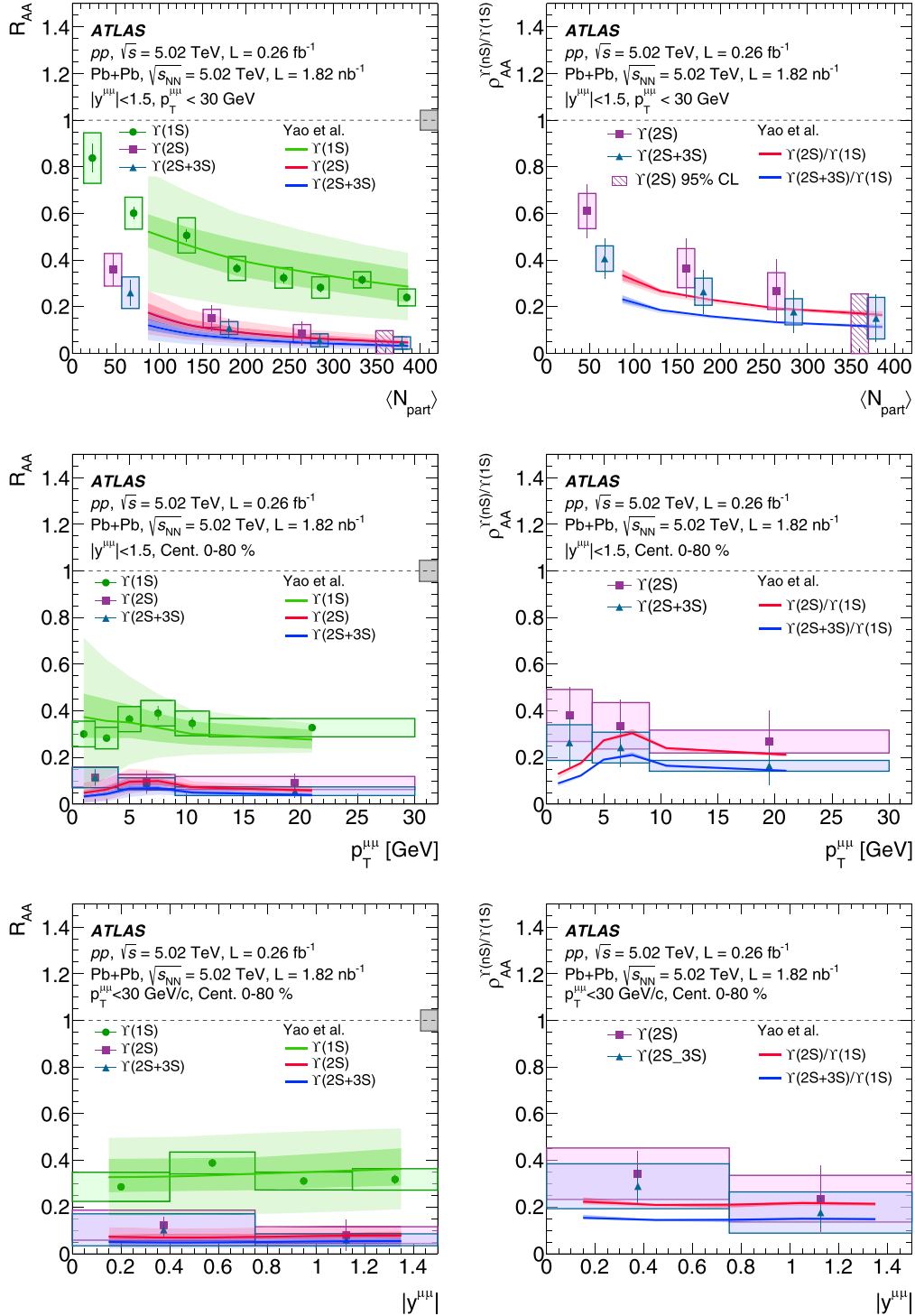
FIG. 7. The nuclear modification factor R_{AA} of \gamma(1S) , \gamma(2S) , and \gamma(2S + 3S) (left column) and the double ratio \rho_{AA}^{\gamma(nS)/\gamma(1S)} for \gamma(2S) and \gamma(2S + 3S) (right column) as functions of centrality (top row), p_T^{\mu\mu} (center row), and rapidity (bottom row) at 5.02 TeV per nucleon-nucleon pair compared to a calculation by Yao et al. [8] (solid curves). Dark color bands show theory uncertainty due to the nucleus parton distribution function choice. Light color bands show model uncertainties due to varying the calculation parameters by \pm 10\% .
