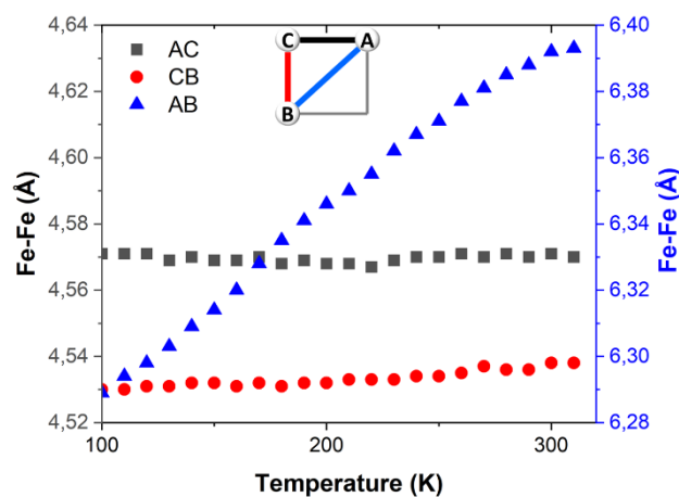
Figure 3. Temperature dependence of the Fe – Fe distances in FE3 . Distances AC and CD share the same axis.
