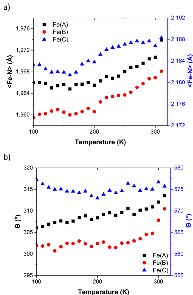
Figure 2. Temperature dependence of a) <Fe-N> bond length distances and b) angular distortions ( \Theta ) in FE3 . Values for Fe(A) and Fe(B) share the same axis.
