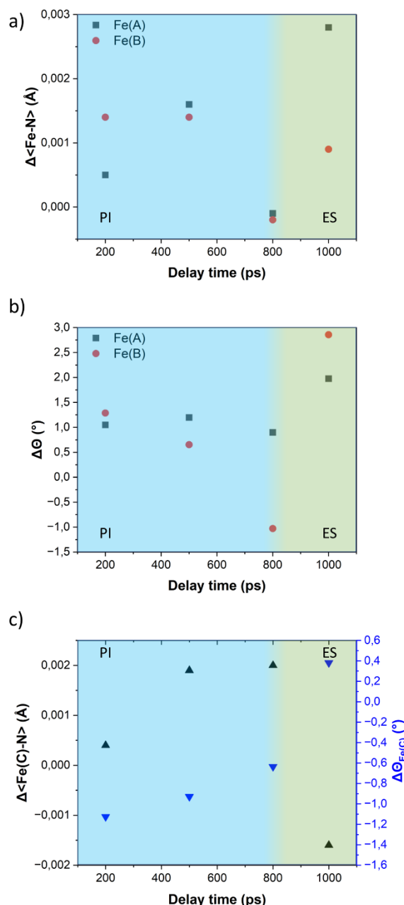
Figure 7. Time-delay dependence of a) \Delta \langle \text{Fe-N} \rangle ; b) \Delta \Theta of the Fe(A) and Fe(B) ions; and c) those from the Fe(C) ion. Photoinduced (PI) and elastic (ES) steps are shown in blue and green background, respectively.
