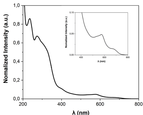
Figure 5. UV-vis spectrum of FE3 grid in acetonitrile. (inset) Enlargement of the 350–800 nm range.
