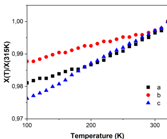
Figure 4. Relative temperature dependence of unit cell parameters of FE3 .
