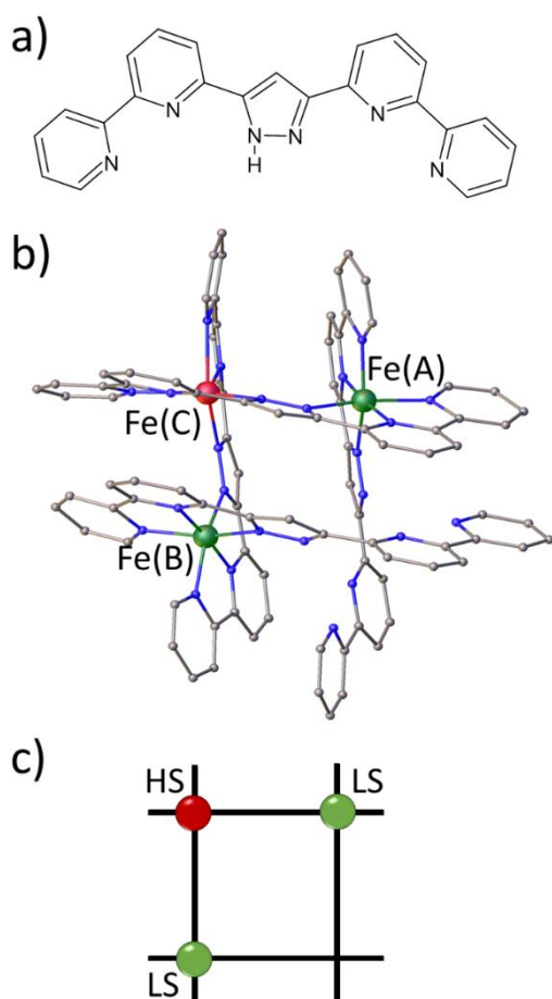
Figure 1. a) Pyrazole-bridged compartmental ligand HL. b) Molecular representation of the [\text{Fe}_3\text{L}_4]^{4+} grid. Fe(A) and Fe(B) ions are in the LS state, and Fe(C) ions are in the HS state. Counter ions, solvent molecules and hydrogen atoms are omitted for clarity. c) Schematic representation of the grid in FE3 .
