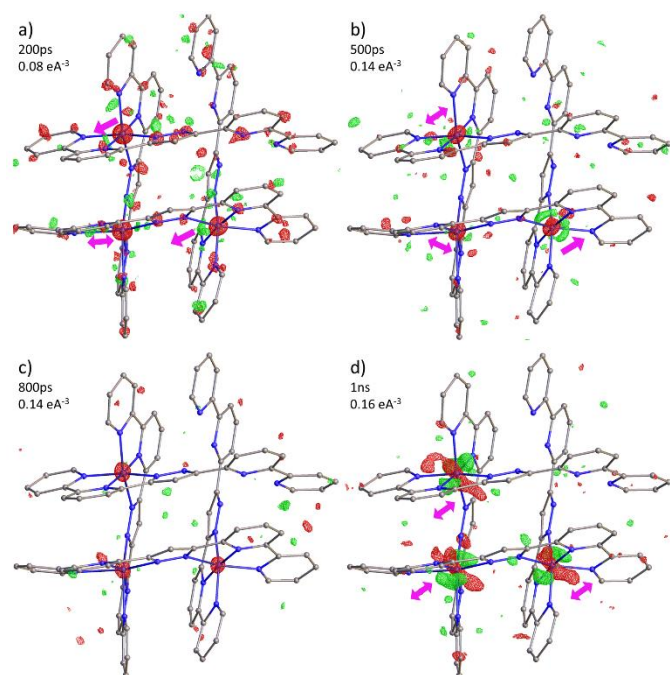
Figure 6. Photodifference maps of FE3 . Isosurfaces (green positive, red negative) and delay times are shown in each figure. Arrows give an approximate direction of the electron density shift.
