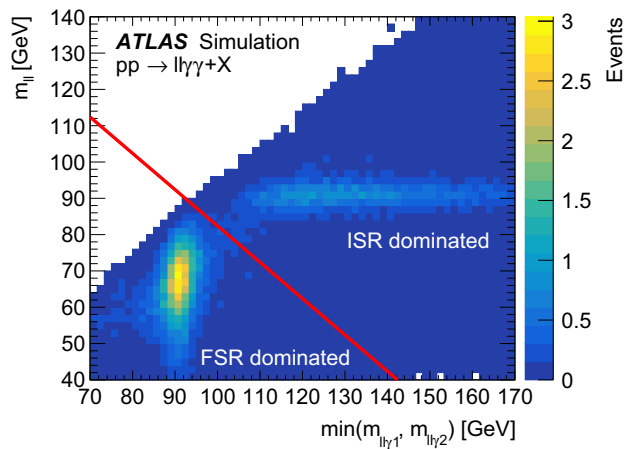
Fig. 2 The predicted detector-level distribution in SHERPA 2.2.10 simulation of the dilepton invariant mass versus the smaller of the two three-body masses formed from the dilepton system and each of the two photons. The events are subject to the full set of signal region requirements, with the exception of the FSR removal selection ( m_{\ell\ell} + \min(m_{\ell\ell\gamma_1}, m_{\ell\ell\gamma_2}) > 2m_Z ). The cut value is indicated by the red line
