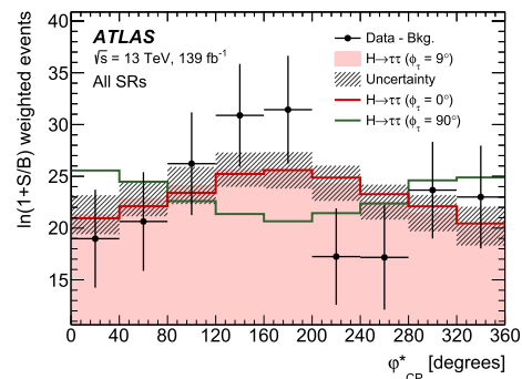
Fig. 7 Combined post-fit distribution of \phi_{CP}^* from all signal regions in both the \tau_{\text{lep}} \tau_{\text{had}} and \tau_{\text{had}} \tau_{\text{had}} channels. Events are weighted with \ln(1 + S/B) for the corresponding signal region. The background is subtracted from data. The best-fit H \rightarrow \tau\tau signal is shown in solid pink, while the red and green lines indicate the predictions for the pure CP -even (scalar, SM) and pure CP -odd (pseudoscalar) hypotheses, respectively, all scaled to the best-fit H \rightarrow \tau\tau signal yield. The hatched uncertainty band includes all sources of uncertainty after the fit to data, and represents the same uncertainty in the total signal and background predictions as in Fig. 4
