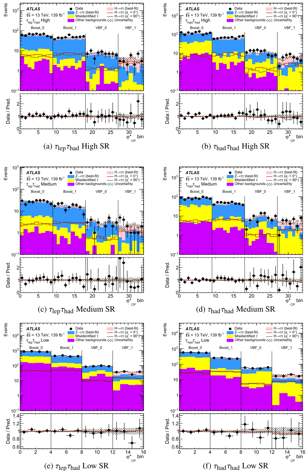
Fig. 4 Post-fit distributions of \phi_{CP}^* in the signal regions (SRs), showing a \tau_{lep} \tau_{had} High SR, b \tau_{had} \tau_{had} High SR, c \tau_{lep} \tau_{had} Medium SR, d \tau_{had} \tau_{had} Medium SR, e \tau_{lep} \tau_{had} Low SR, and f \tau_{had} \tau_{had} Low SR. The \phi_{CP}^* bins are counted incrementally through all VBF and Boost categories and cover the range [0, 360]^\circ for each category. The best-fit H \rightarrow \tau\tau signal is shown in solid pink, while the red and green lines indicate the predictions for the pure CP -even (scalar, SM) and pure CP -odd (pseudoscalar) hypotheses, respectively, scaled to the predicted signal yield. ‘Other backgrounds’ include W , diboson, top, Z \rightarrow \ell\ell and H \rightarrow WW^* . The hatched uncertainty band includes all sources of uncertainty after the fit to data
