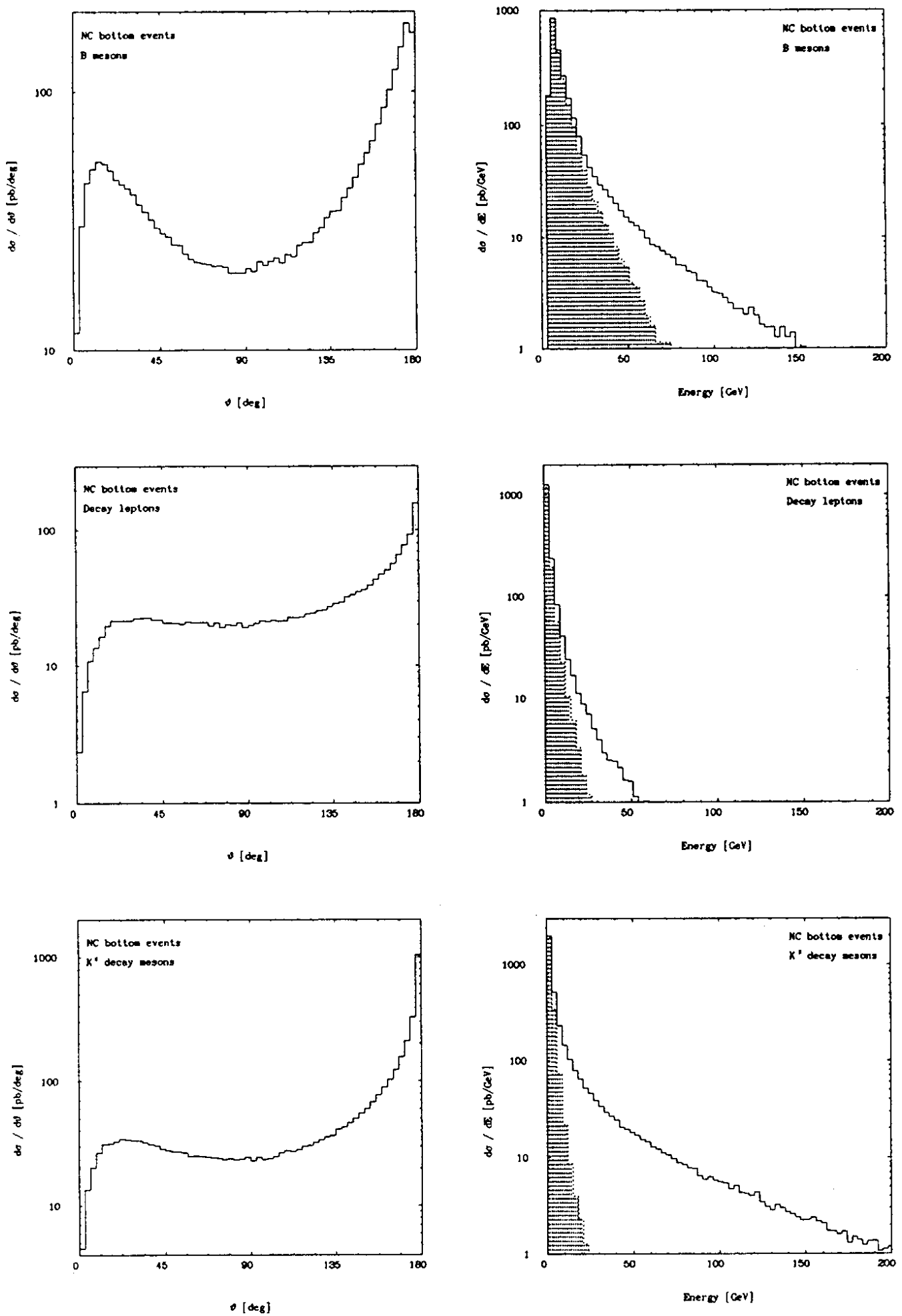
Figure 4.5 Energy and polar angle distributions for B mesons, decay kaons and leptons, produced in the NC process ep \rightarrow e\bar{b}\bar{b}X and subsequent bottom decays calculated at HERA energy \sqrt{s} = 314 \text{ GeV} . The energy distributions resulting after imposing a beam pipe cut of 100 mrad are represented by the shaded areas. (From ref. [60])
