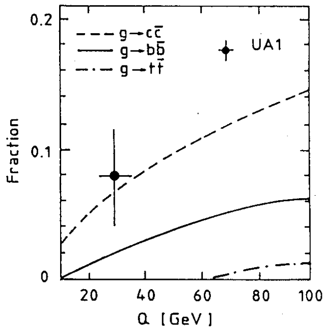
Figure 2.4 Perturbative estimates of heavy quark fraction in a gluon jet in pp/p\bar{p} as a function of the parton-parton c.m.s. energy Q compared with the UA1 data [2]. Theoretical curves are from Müller and Nason in ref. [37].
