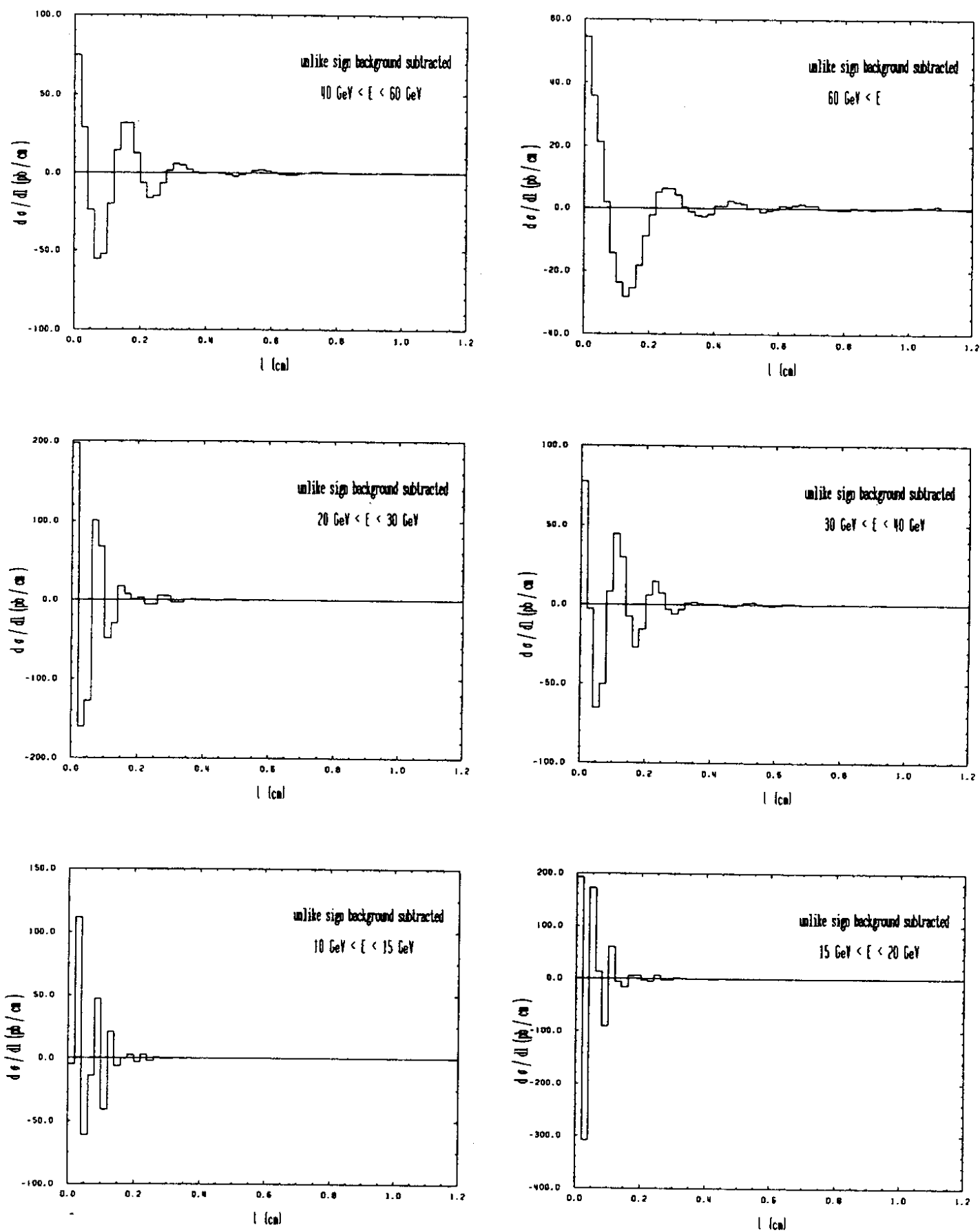
Figure 4.31 Same as Fig. 4.30 but with x_s = 10 .
