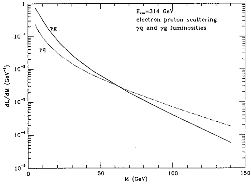
Figure 2.5 Luminosity functions for initial parton combinations \gamma g and \gamma q in ep collisions at \sqrt{s} = 314 GeV. M denotes the subenergy of the parton collisions. (From ref. [29]).
