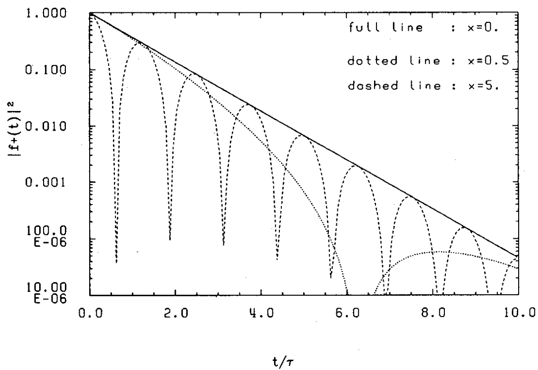
Figure 4.21 The function |f_+(t)|^2 as defined in (4.57), for x = 0.5, 5, 0 .
