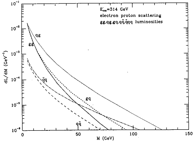
Figure 2.6 Luminosity functions for gg , gq , qg , \bar{q}q and q\bar{q} parton collisions in electron proton scattering at HERA energy, \sqrt{s} = 314 GeV (From ref. [29]).
