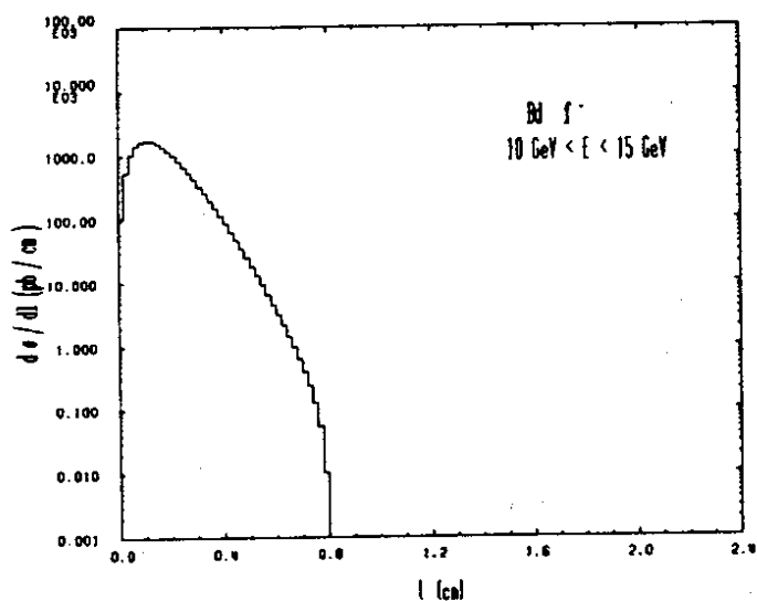
Figure 4.24 Same as Fig. 4.23 but for the "wrong sign meson" B_d^0 \rightarrow \bar{B}_d^0 with x_d = 0.5 .
