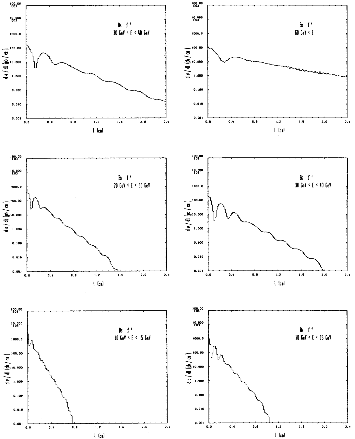
Figure 4.25 Distribution in decay length, d\sigma/dl , for the "right sign meson" B_s^0 \rightarrow B_s^0 with x_s = 5.0 in the process ep \rightarrow ebb\bar{X} \rightarrow B_s X .
