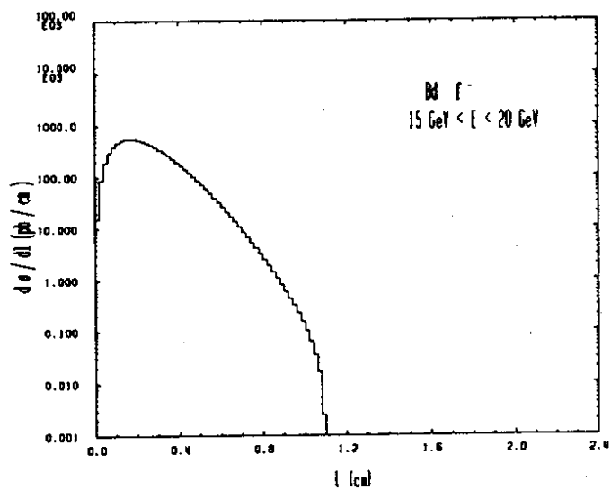
Figure 4.24 Same as Fig. 4.23 but for the "wrong sign meson" B_d^0 \rightarrow \bar{B}_d^0 with x_d = 0.5 .
