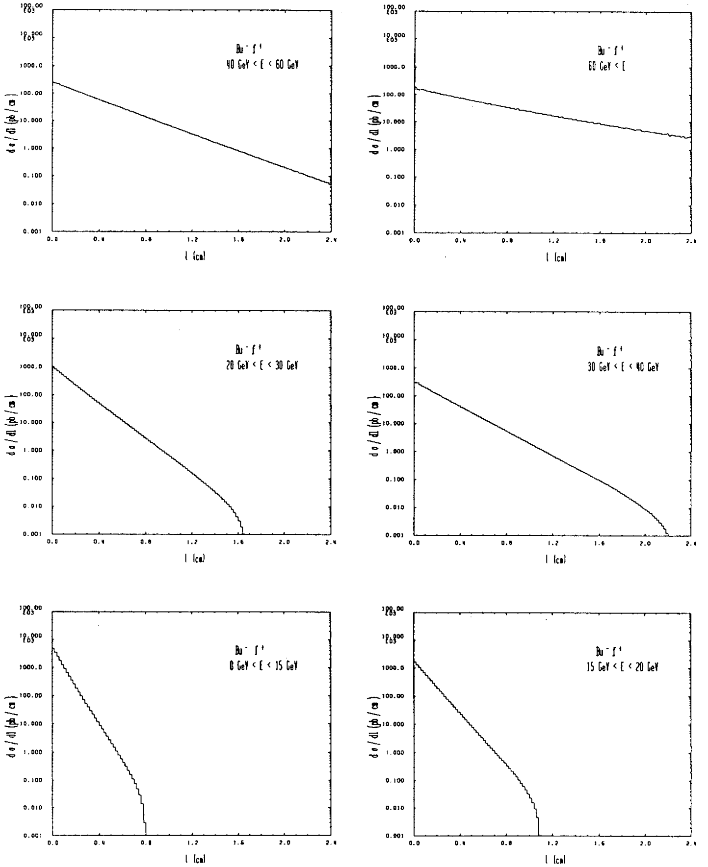
Figure 4.29 Distribution in decay length \frac{d\sigma}{dl} for the process ep \rightarrow e\bar{b}bX \rightarrow B_u^- X at HERA energy \sqrt{s} = 314 GeV, for the various indicated bins in E_{B_u^-} . (From ref. [60])
