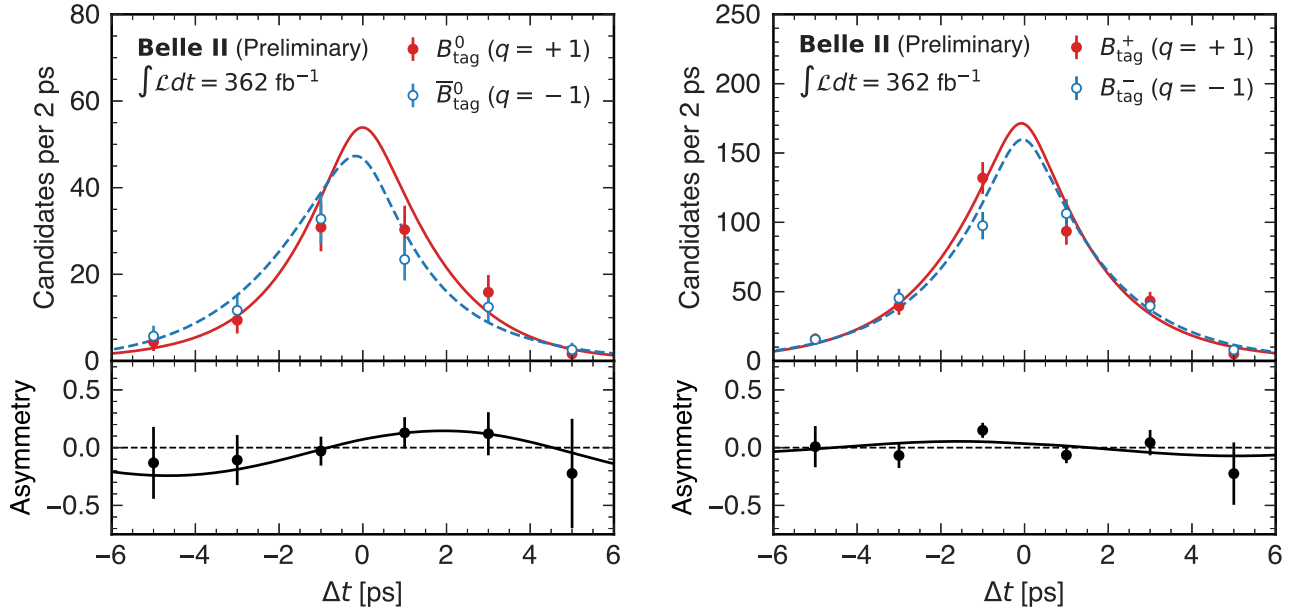
Figure 3: Distributions, and fit projections, of \Delta t for flavor-tagged (left) B^0 \rightarrow \phi K_S^0 and (right) B^+ \rightarrow \phi K^+ candidates subtracted of the continuum background. The fit PDFs corresponding to q = -1 and q = +1 tagged distributions are shown as dashed and solid curves, respectively. The yield asymmetries, defined as (N(q = +1) - N(q = -1)) / (N(q = +1) + N(q = -1)) , are displayed in the bottom subpanels.
