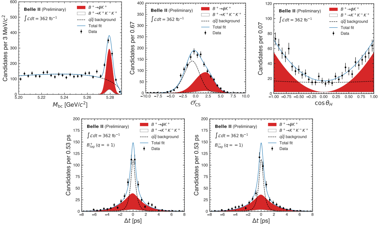
Figure 1: Distributions of (top left) M_{bc} , (top center) \mathcal{O}'_{CS} , (top right) \cos\theta_H , (bottom left) \Delta t for B^+ -tagged and (bottom right) \Delta t for B^- -tagged B^+ \rightarrow \phi K^+ candidates (data points) with fits overlaid (curves and stacked shaded areas). The M_{bc} distribution is displayed for candidates with \mathcal{O}'_{CS} > -1 and the \mathcal{O}'_{CS} distribution is displayed for candidates with M_{bc} > 5.27 \text{ GeV}/c^2 . The \cos\theta_H and \Delta t distributions are displayed for candidates with \mathcal{O}'_{CS} > -1 and M_{bc} > 5.27 \text{ GeV}/c^2 .
